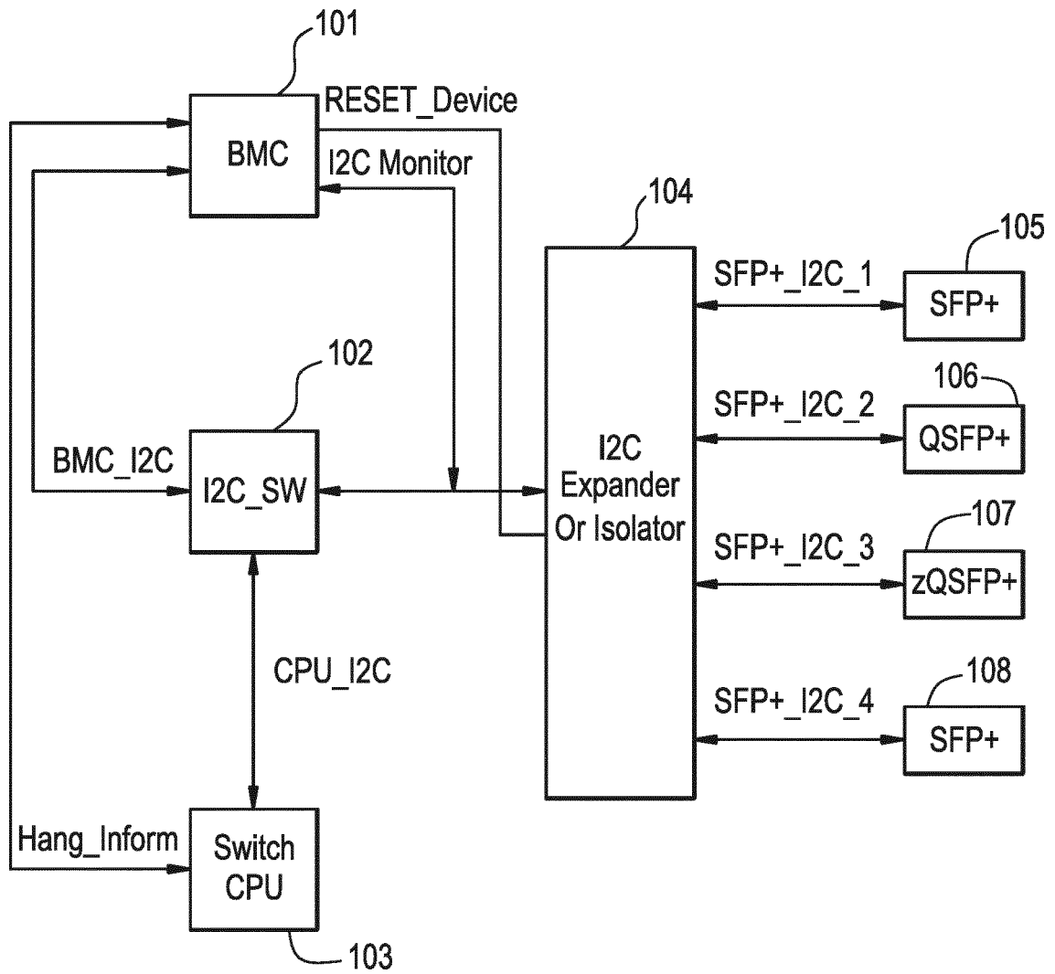
FIG. 1 PRIOR ART
