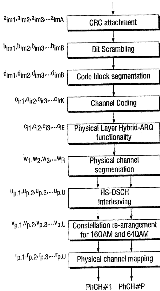
FIG. 4 (Prior Art)
