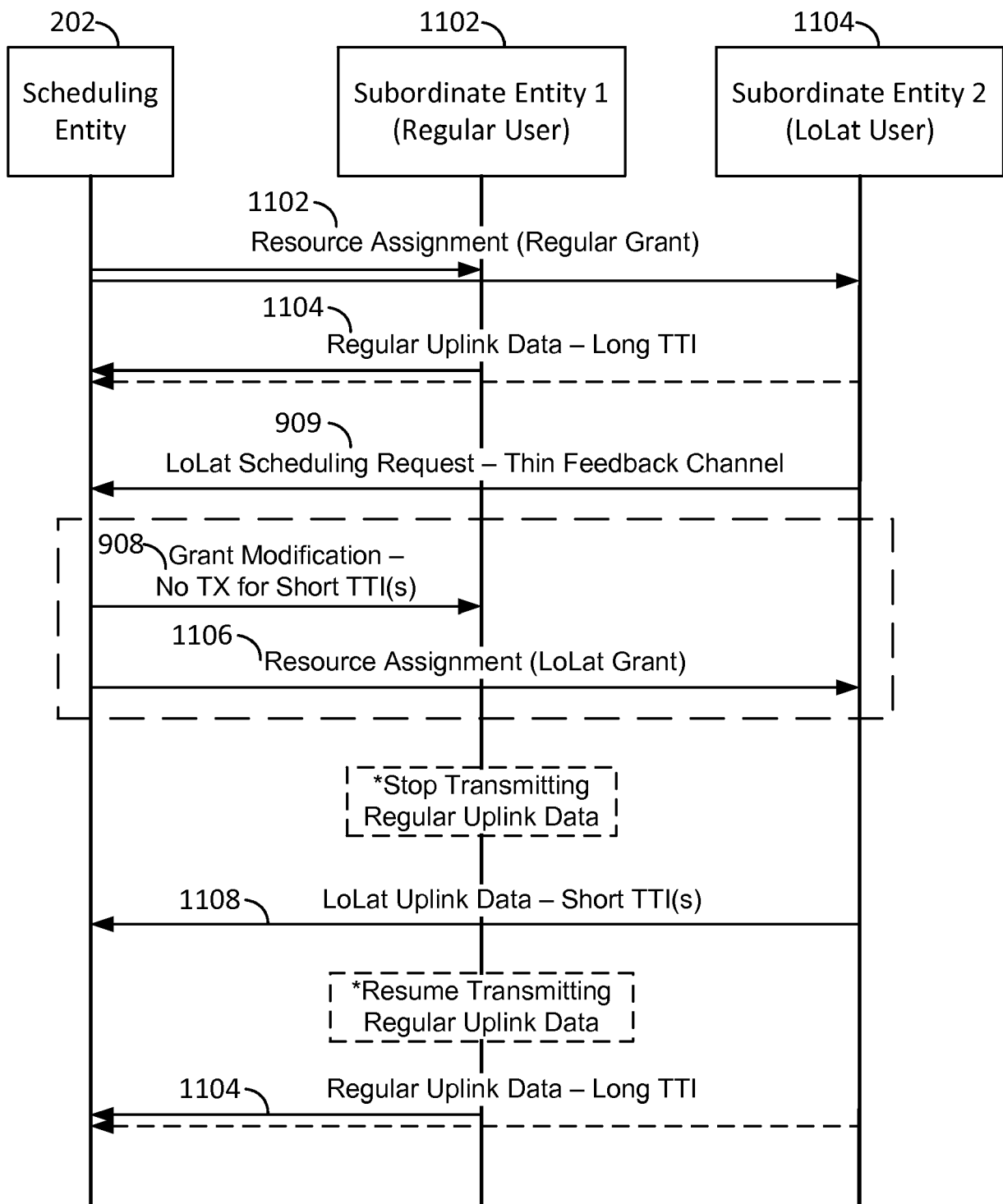
FIG. 11 UL/UL Multiplexing
