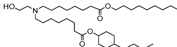
(Compound 188),
