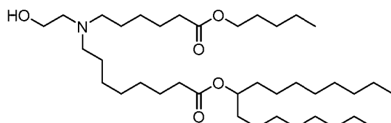
(Compound 104),
