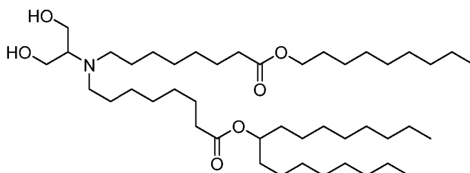
(Compound 156),
