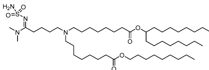
(Compound 219),
