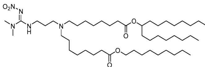
(Compound 209),
