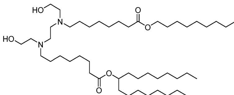
(Compound 159),
