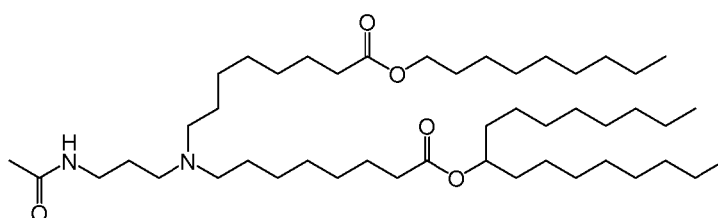
(Compound 108),
