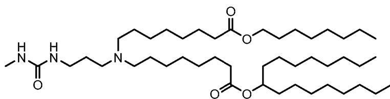
(Compound 41),
