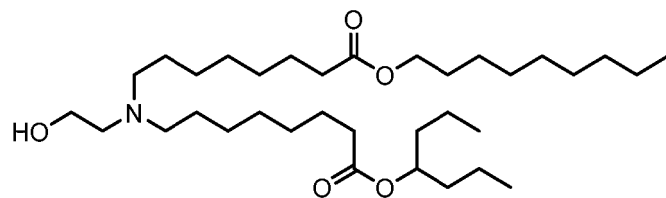
(Compound 58),
