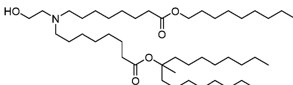
(Compound 82),
