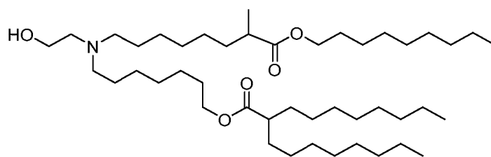
(Compound 163),
