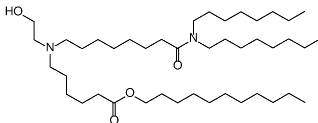
(Compound 129),
