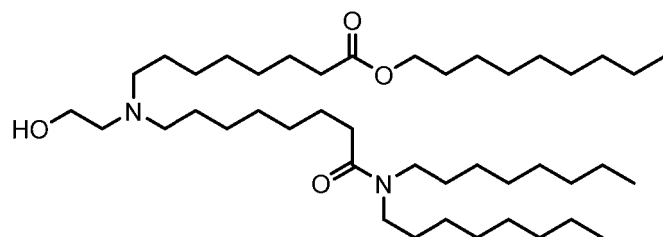
(Compound 144),
