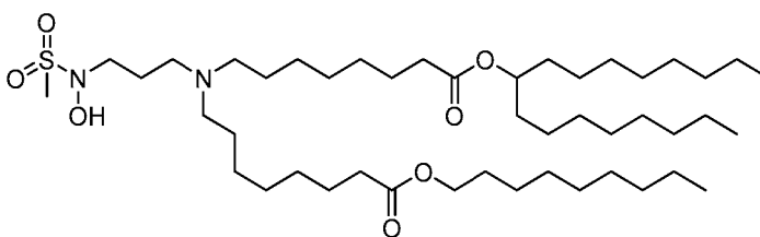
(Compound 206),
