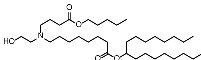
(Compound 52),
