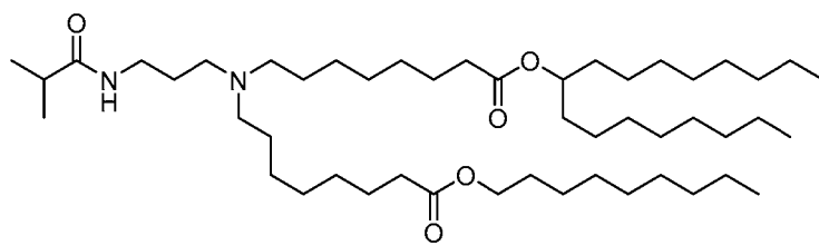
(Compound 194),
