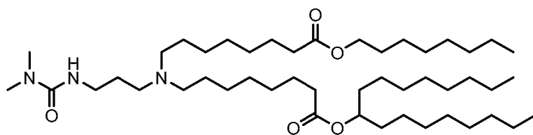
(Compound 39),
