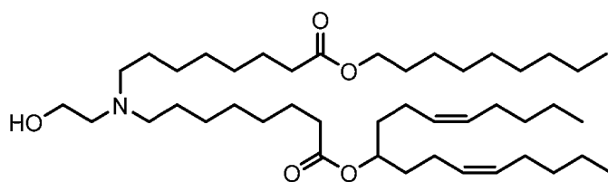
(Compound 60), and
