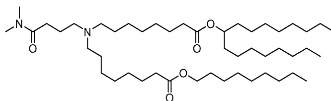
(Compound 224),
