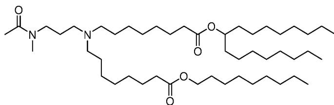
(Compound 196),
