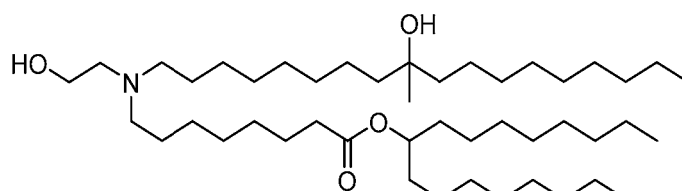
(Compound 171),
