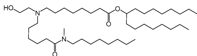
(Compound 146),
