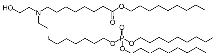
(Compound 127),
