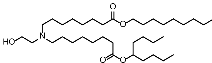
(Compound 57),
