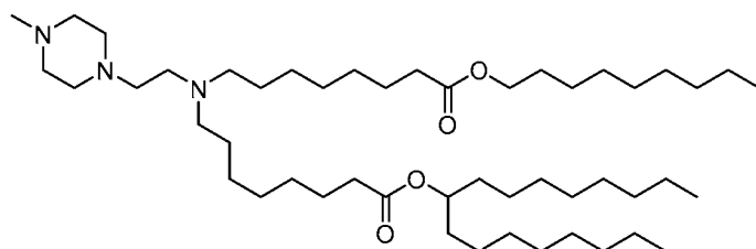
(Compound 101),
