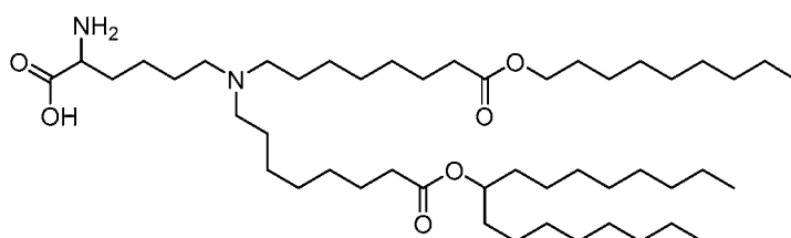
(Compound 106),
