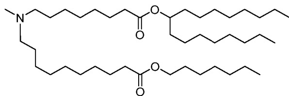
(Compound 149),
