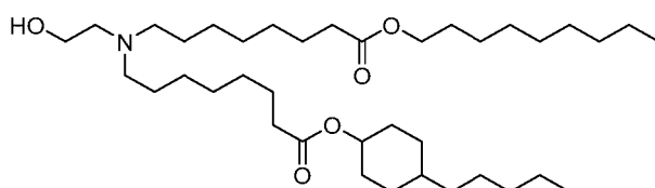
(Compound 79),
