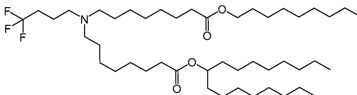
(Compound 107),
