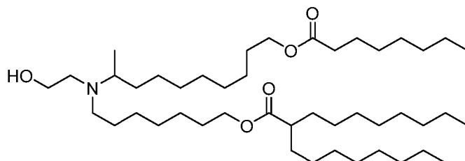
(Compound 162),
