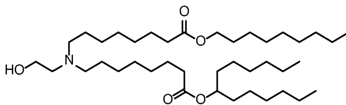
(Compound 56),
