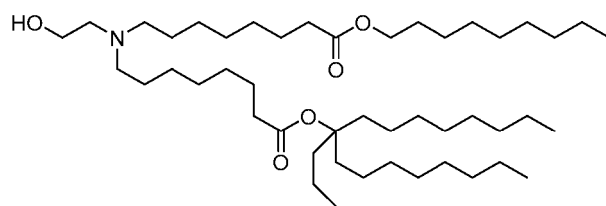
(Compound 84),
