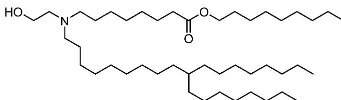
(Compound 153),
