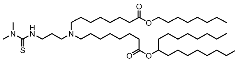
(Compound 40),
