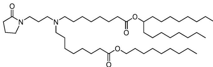
(Compound 195),
