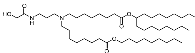
(Compound 198),
