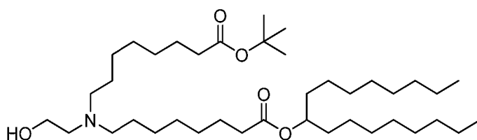
(Compound 155),
