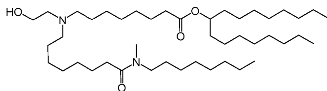
(Compound 145),
