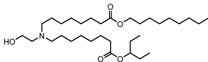
(Compound 59),
