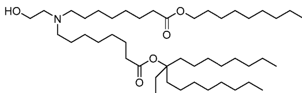
(Compound 83),
