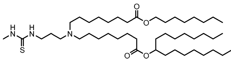
(Compound 42),
