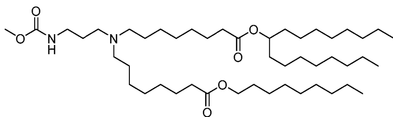
(Compound 181),
