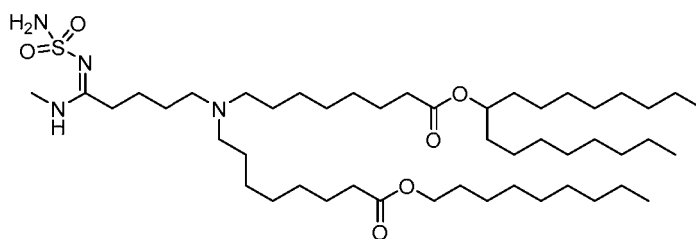
(Compound 220),
