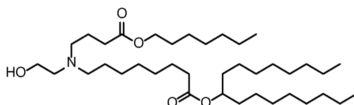
(Compound 54),
