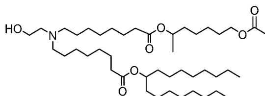
(Compound 214),
