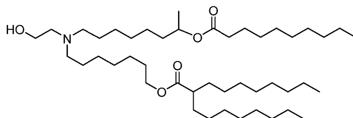
(Compound 165),
