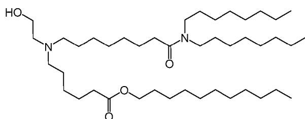
(Compound 129),
