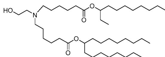
(Compound 91),
