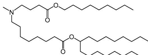
(Compound 126),
