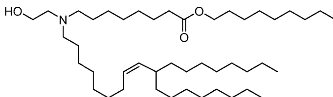
(Compound 152),
