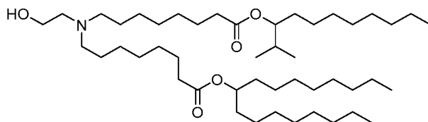
(Compound 78),
