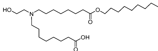
(Compound 167),
