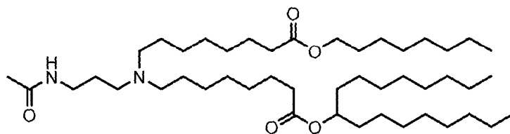
(Compound 37),
