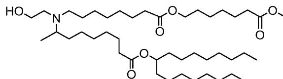
(Compound 192),
