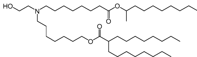
(Compound 135),
