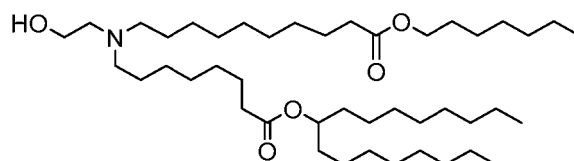
(Compound 189),
