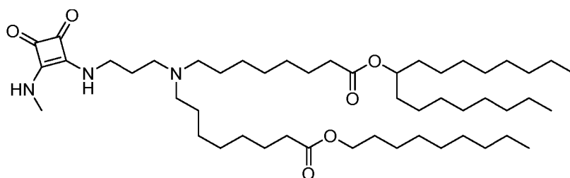
(Compound 182),
