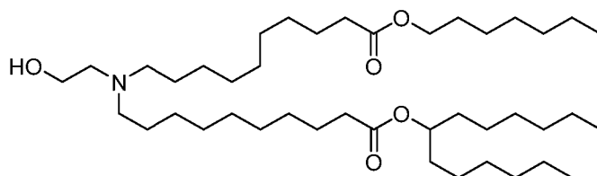
(Compound 186),
