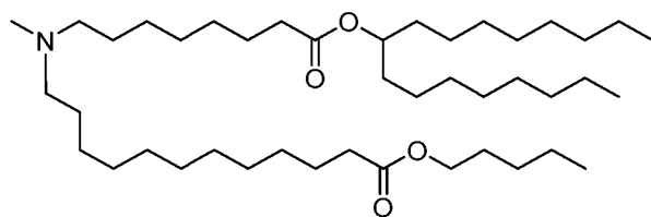
(Compound 150),
