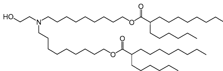
(Compound 133),
