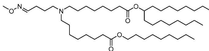
(Compound 229),
