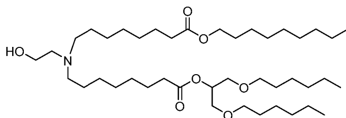
(Compound 183),
