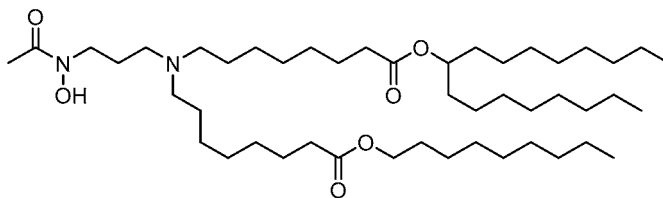
(Compound 204),
