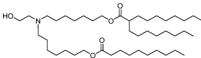
(Compound 151),
