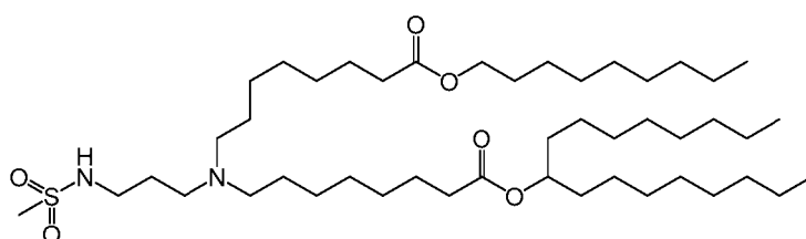
(Compound 109),
