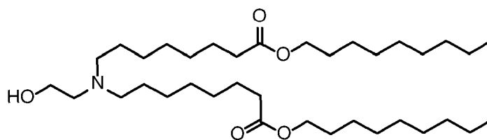
(Compound 138),
