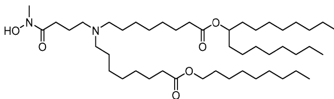
(Compound 227),
