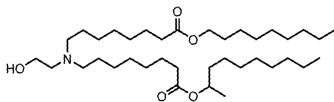
(Compound 36),
