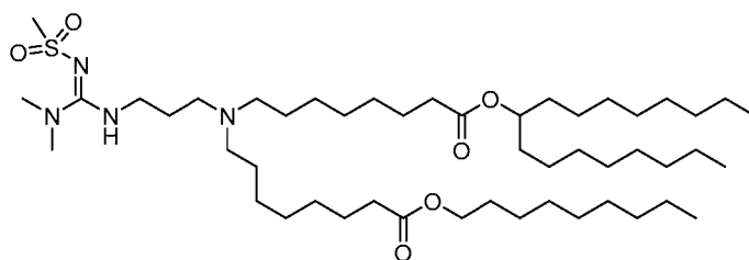
(Compound 213),
