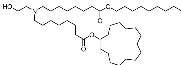
(Compound 81),
