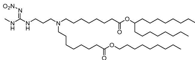
(Compound 200),
