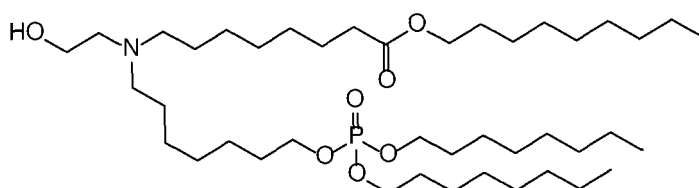
(Compound 131),
