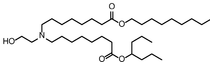
(Compound 58),
