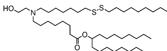
(Compound 215),
