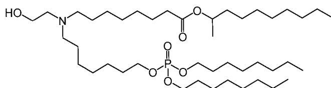
(Compound 132),
