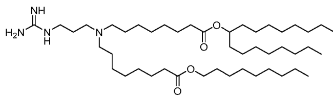
(Compound 207),
