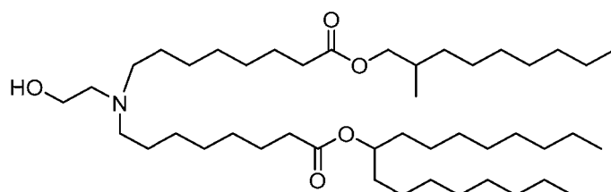
(Compound 184),
