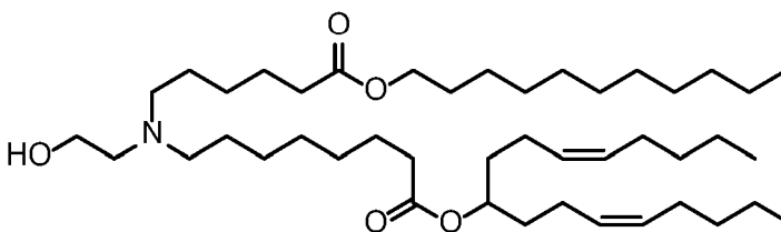
(Compound 61);
