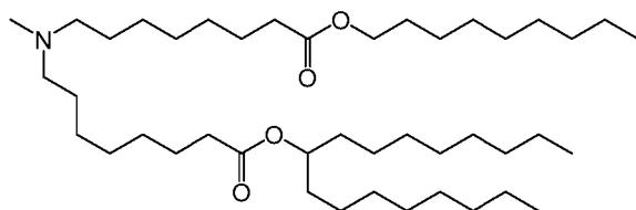
(Compound 123),
