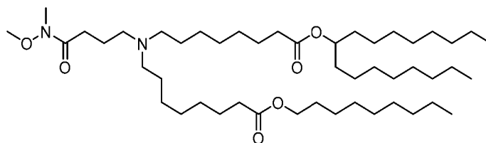
(Compound 228),
