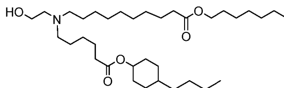
(Compound 191),
