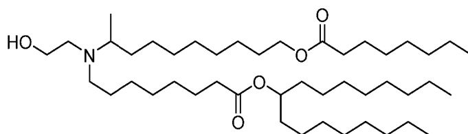
(Compound 161),
