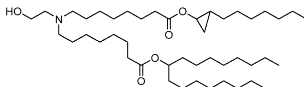
(Compound 88),
