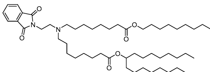
(Compound 100),
