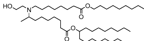
(Compound 217),
