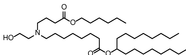
(Compound 53),
