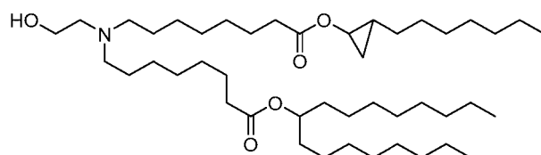
(Compound 93),
