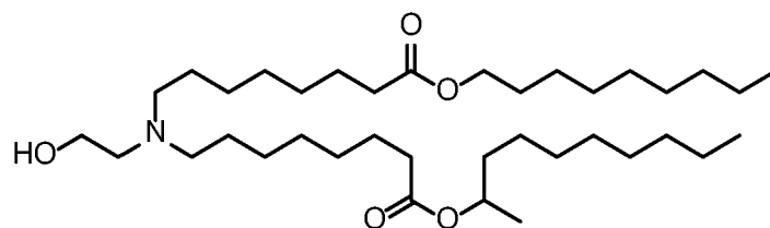
(Compound 36),
