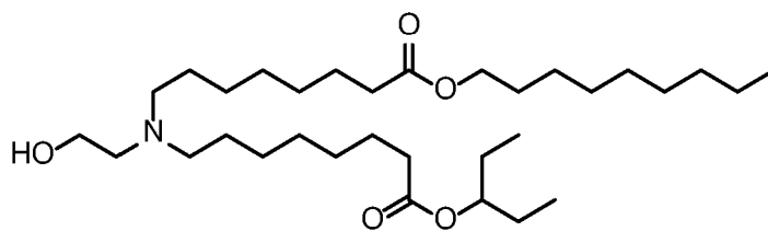
(Compound 59),
