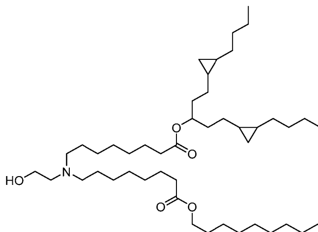
(Compound 160),
