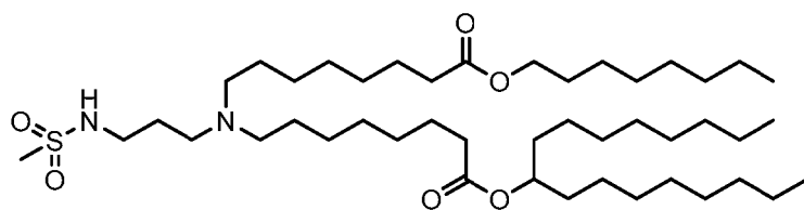
(Compound 38),
