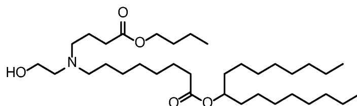
(Compound 51),
