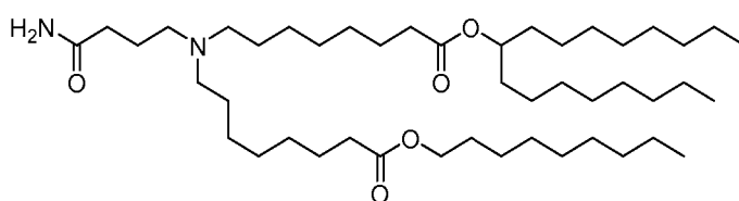
(Compound 222),
