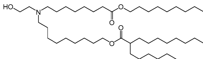
(Compound 134),
