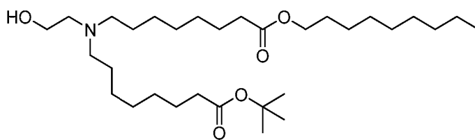
(Compound 158),
