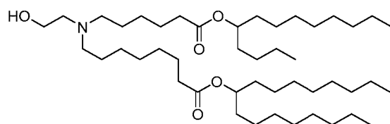
(Compound 77),
