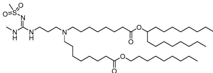
(Compound 212),
