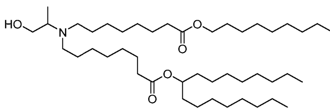
(Compound 157),
