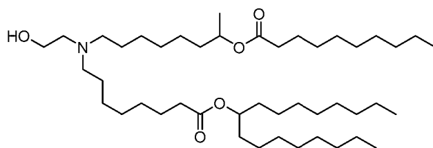
(Compound 98),
