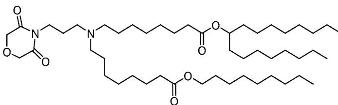
(Compound 202),
