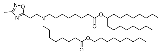
(Compound 230),
