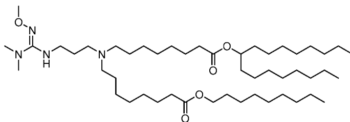
(Compound 211),
