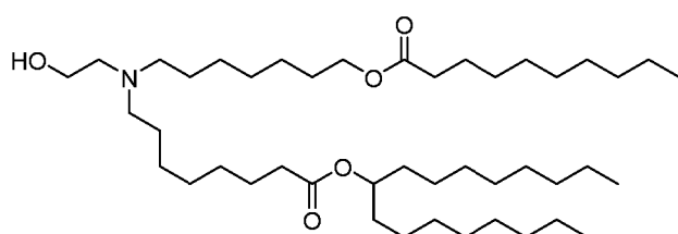
(Compound 96),
