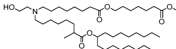
(Compound 190),
