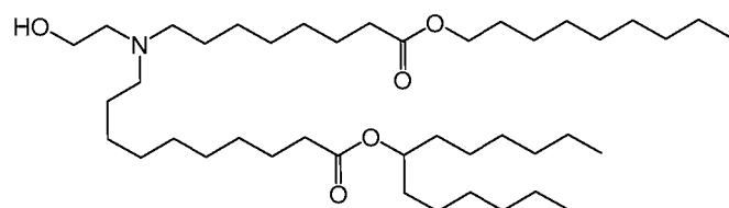
(Compound 147),
