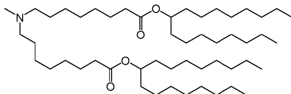
(Compound 124),
