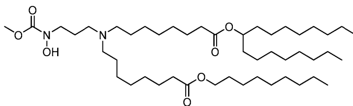
(Compound 205),
