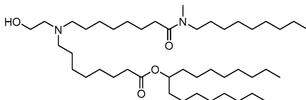
(Compound 105),
