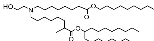
(Compound 216),
