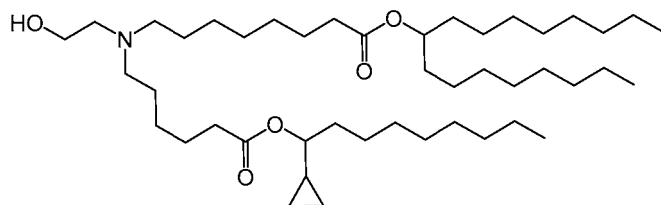
(Compound 128),
