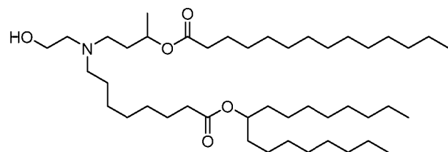
(Compound 99),
