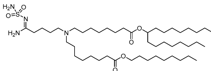
(Compound 221),
