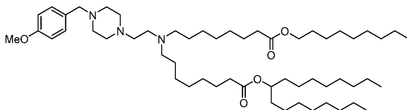
(Compound 102),
