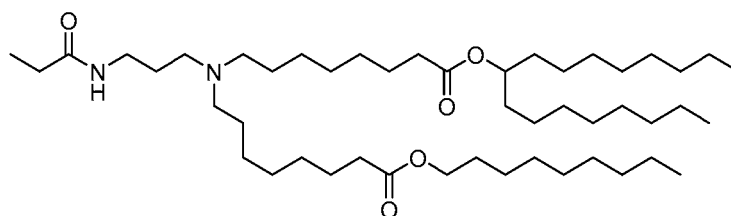
(Compound 193),
