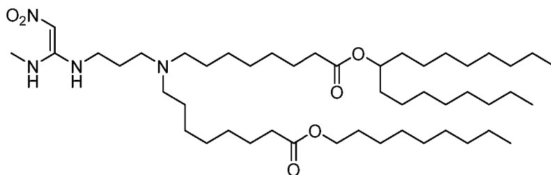
(Compound 170),
