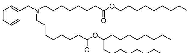
(Compound 94),
