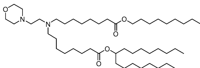
(Compound 103),
