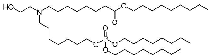
(Compound 131),
