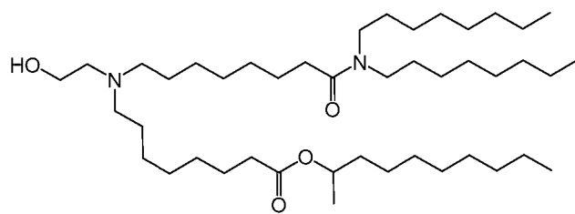
(Compound 130),
