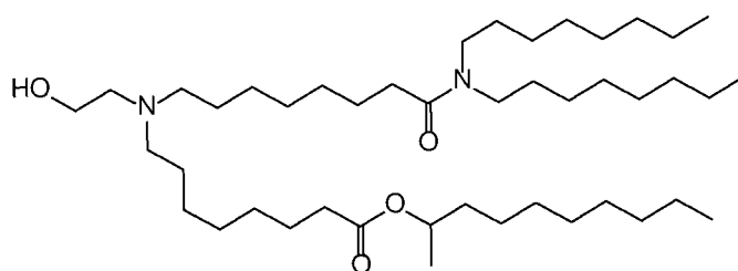
(Compound 130),
