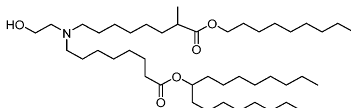
(Compound 164),
