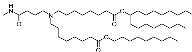
(Compound 223),
