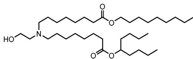
(Compound 57),
