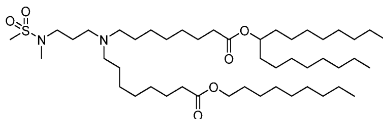
(Compound 173),
