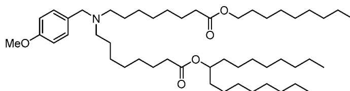
(Compound 95),
