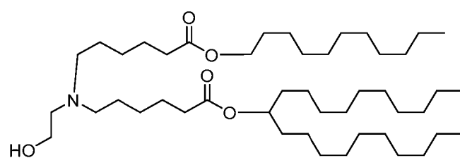
(Compound 185),
