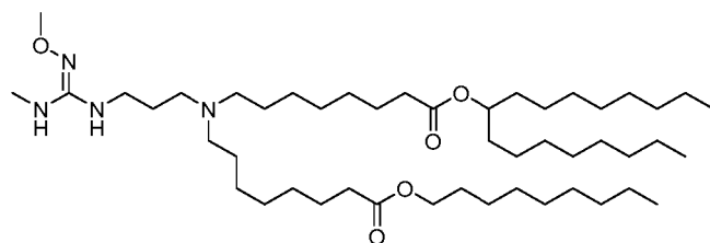
(Compound 210),
