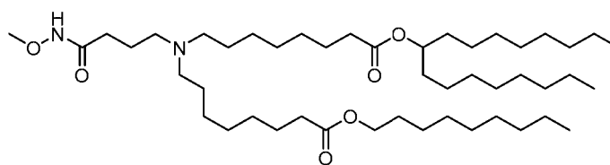
(Compound 226),
