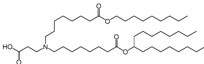
(Compound 125),
