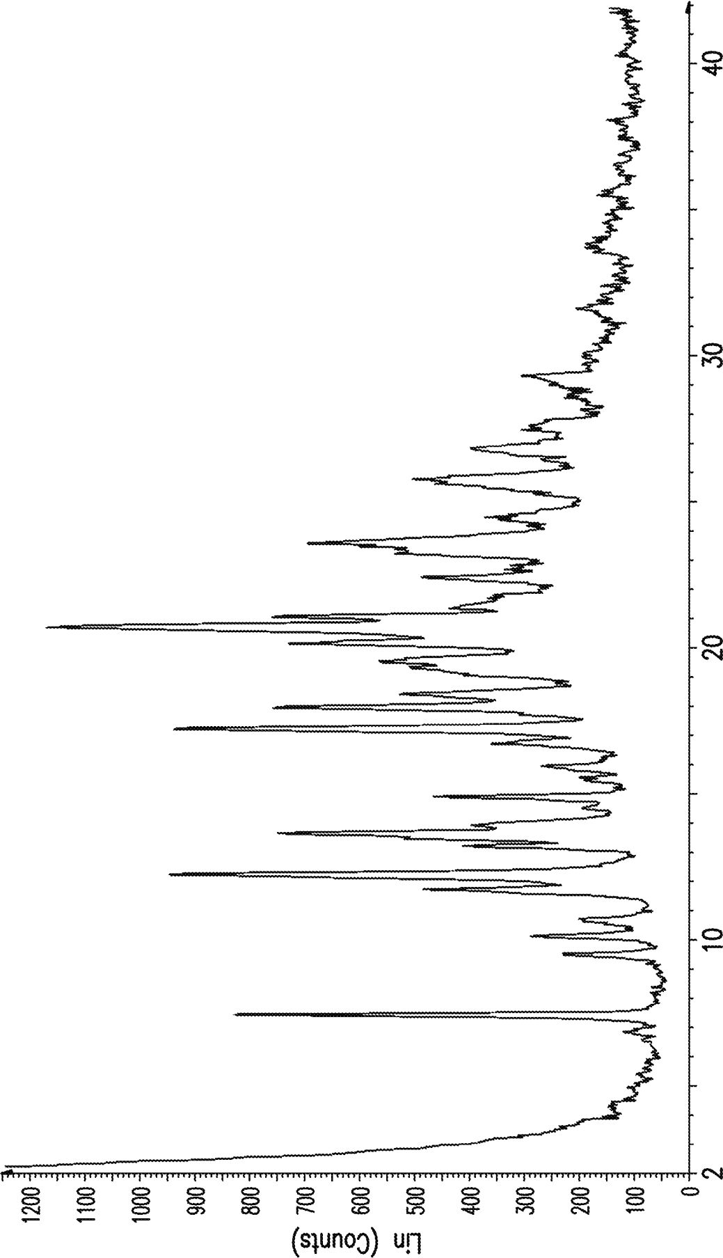
2-Theta-Scale FIG. 18
