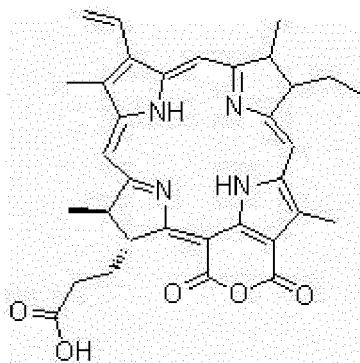
Purpurin 18
