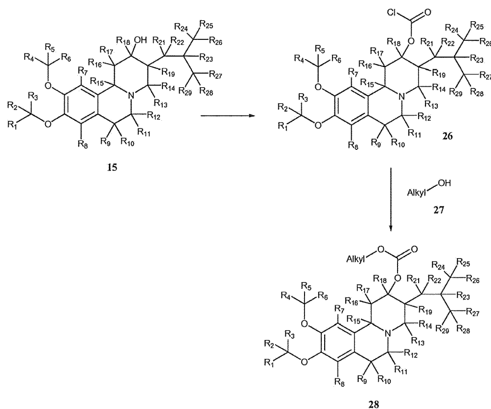
Scheme IV
