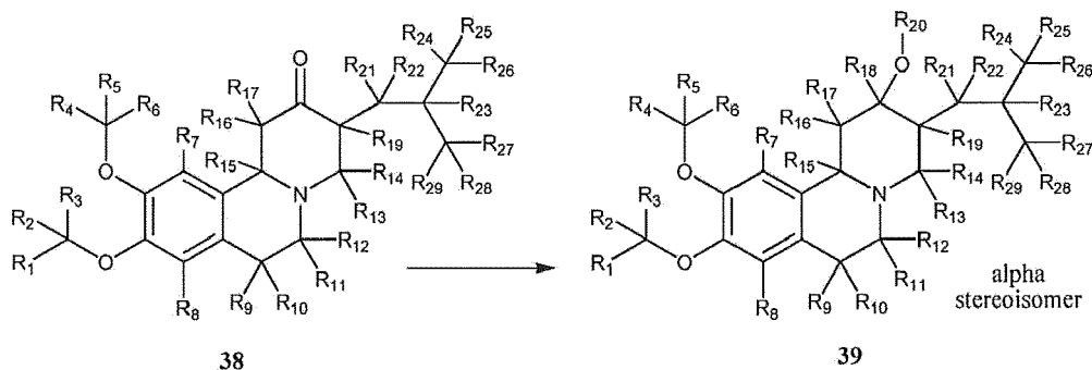
Scheme VIII
