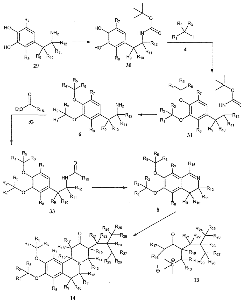
Scheme V
