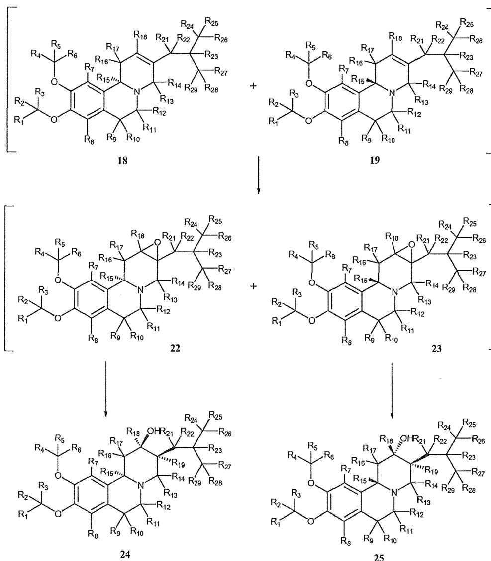
Scheme III
