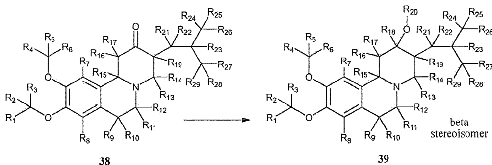
Scheme IX
