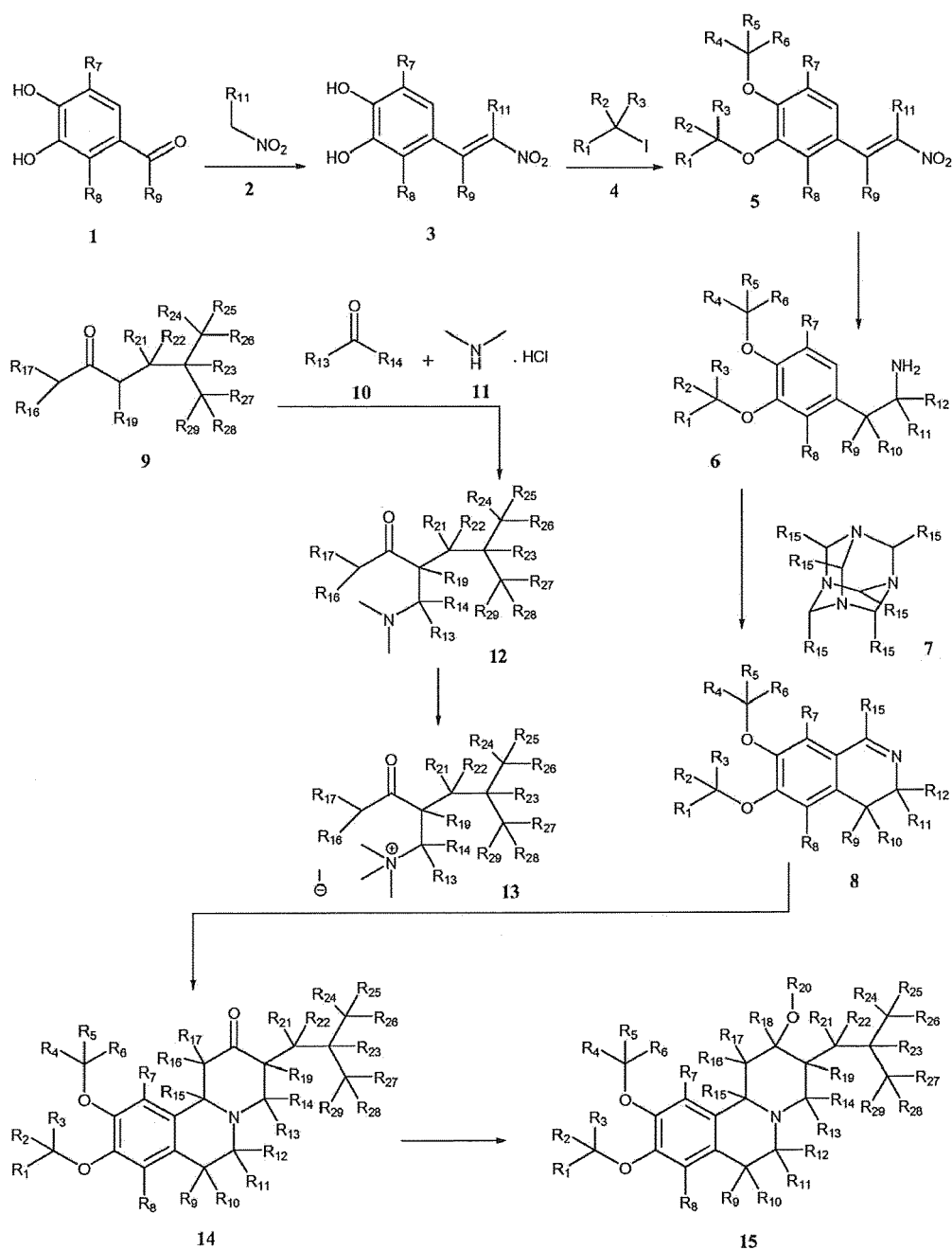
Scheme I
