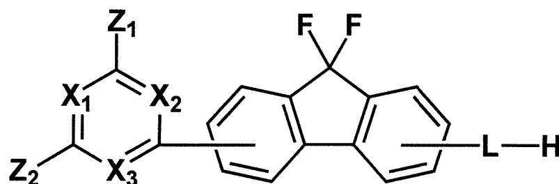
[Chemical Formula 4]
