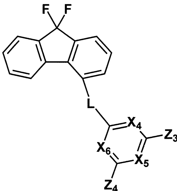
[Chemical Formula 16]
