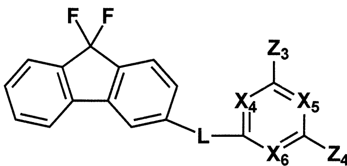
[Chemical Formula 15]
