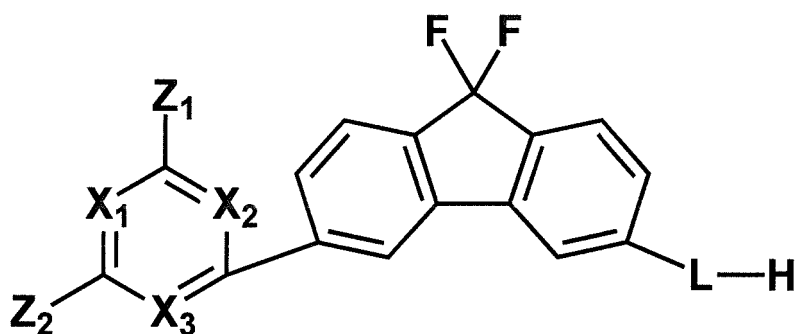
[Chemical Formula 11]
