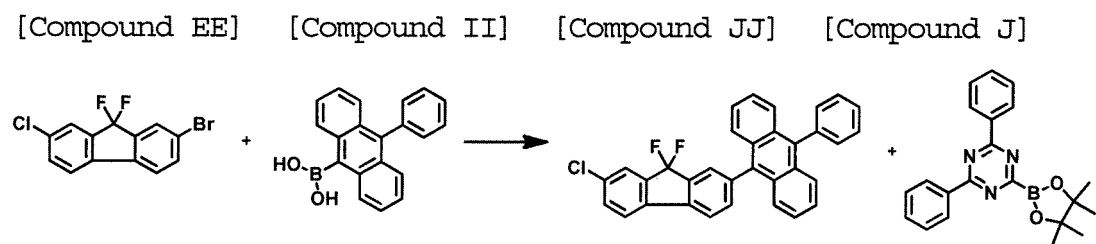
[Compound 20]
