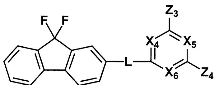
[Chemical Formula 15]
