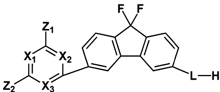
[Chemical Formula 11]
