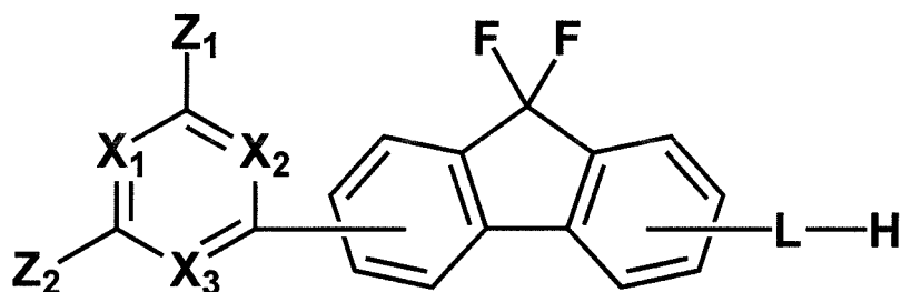
[Chemical Formula 3]
