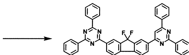
[Compound 19]
