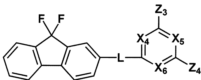
[Chemical Formula 14]
