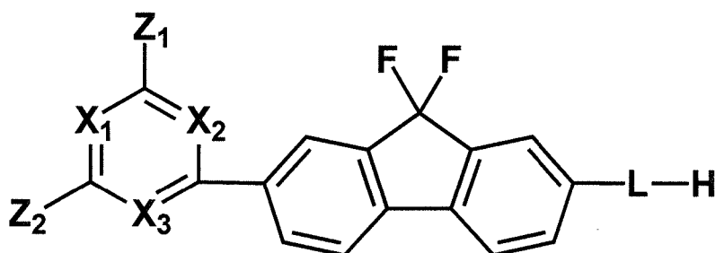
[Chemical Formula 10]
