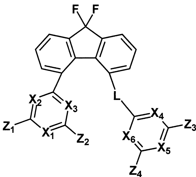
[Chemical Formula 8]
