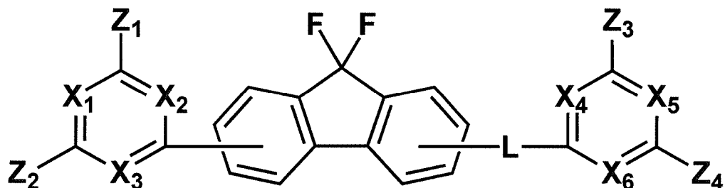
[Chemical Formula 3]
