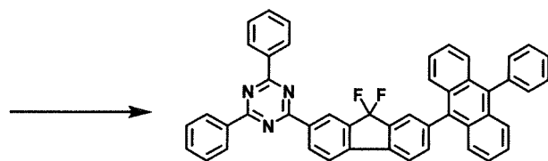
[Compound 20]
