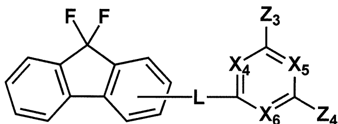
[Chemical Formula 4]
