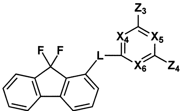
[Chemical Formula 13]
