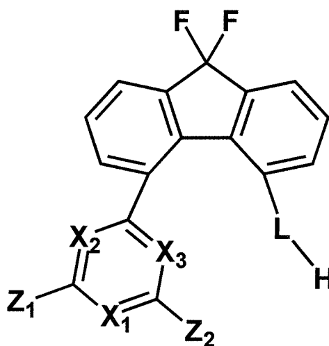
[Chemical Formula 12]
