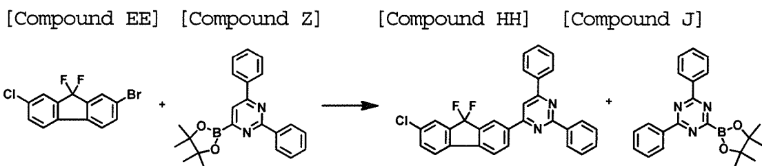
[Compound 19]
