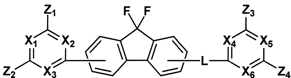
[Chemical Formula 2]
