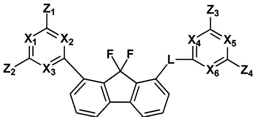
[Chemical Formula 6]
