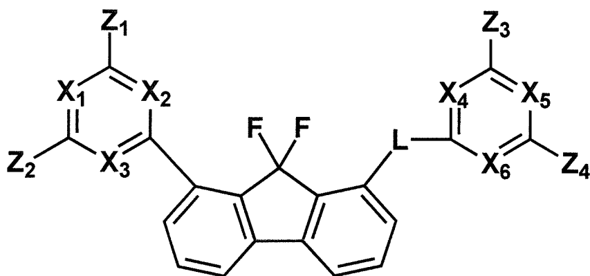
[Chemical Formula 6]
