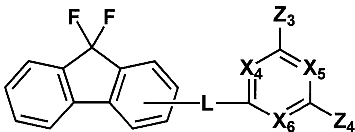
[Chemical Formula 4]
