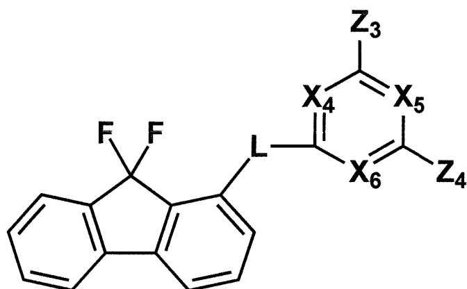
[Chemical Formula 13]
