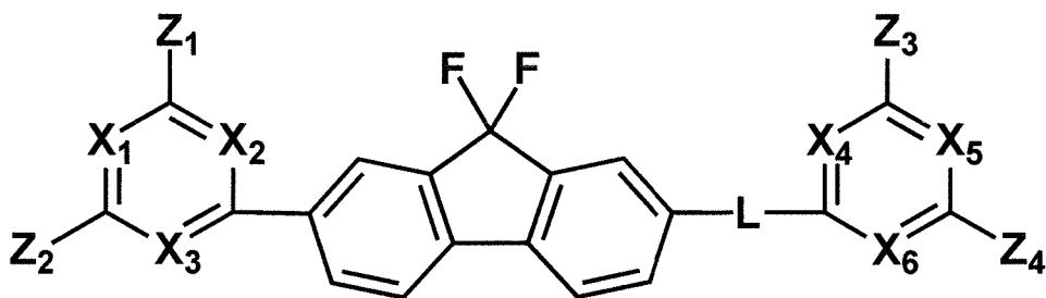
[Chemical Formula 6]
