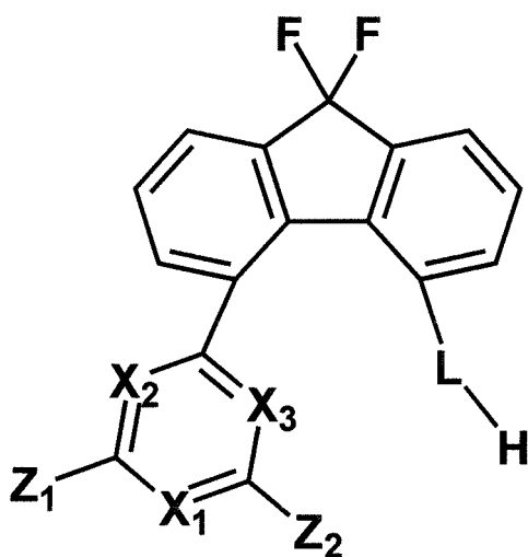
[Chemical Formula 12]
