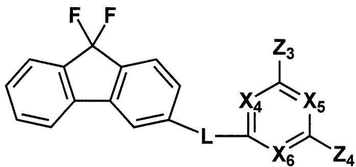
[Chemical Formula 15]
