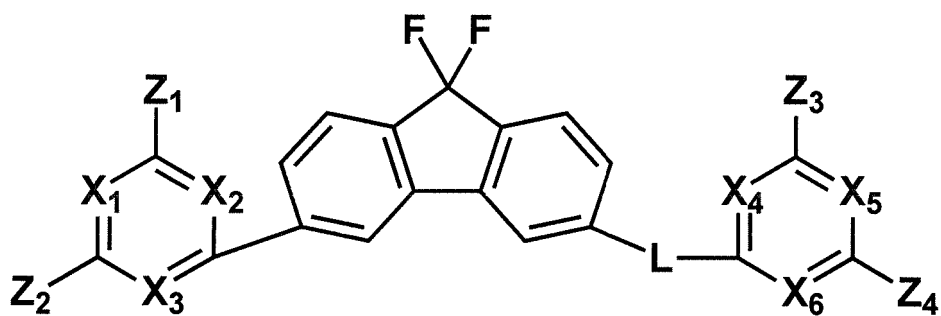
[Chemical Formula 7]
