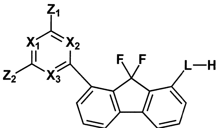
[Chemical Formula 9]
