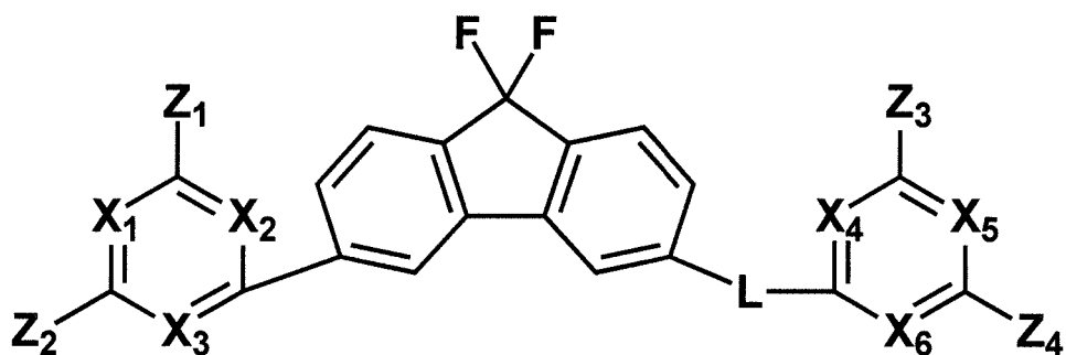
[Chemical Formula 8]
