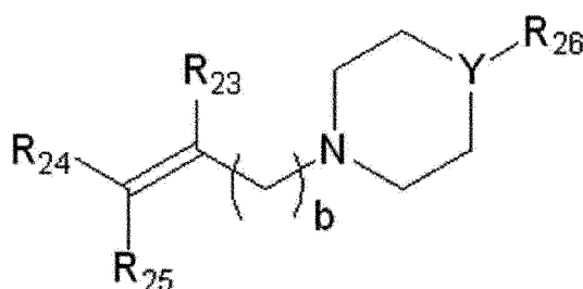
[Formula 2]
