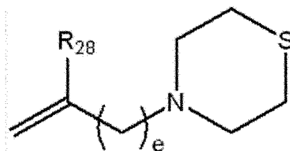
[Formula 27]
