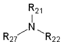
[Formula 11]
