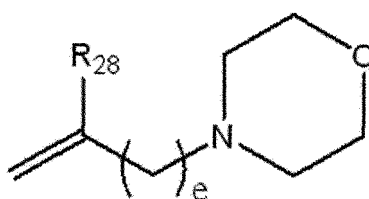
[Formula 25]
