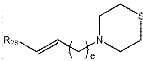
[Formula 27]
