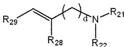
[Formula 14]
