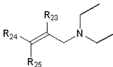
[Formula 7]
