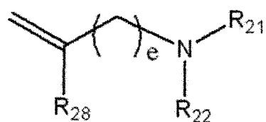
[Formula 19]
