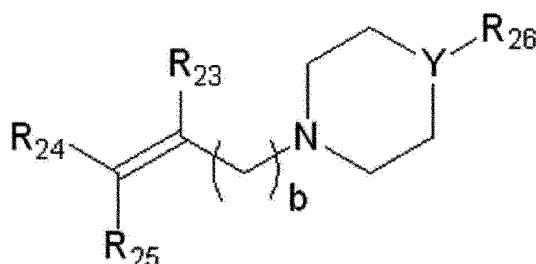
[Formula 2]
