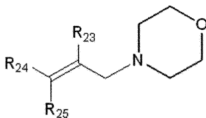
[Formula 8]
