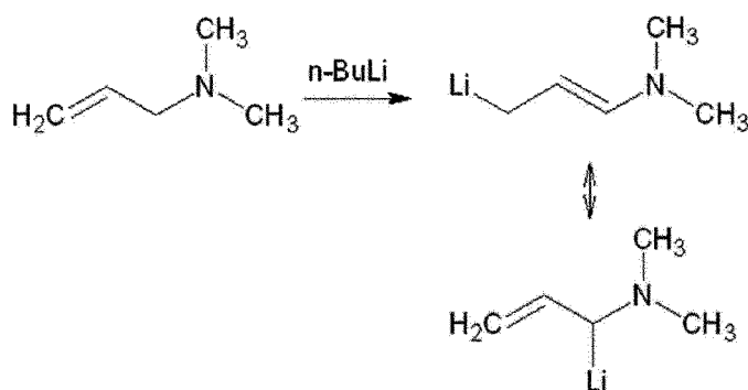
[Reaction Scheme 1]
