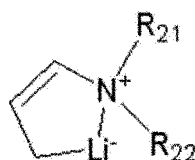
[Formula 12]
