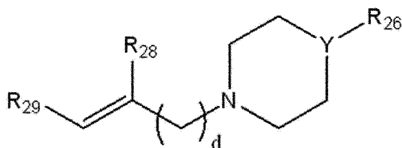
[Formula 16]
