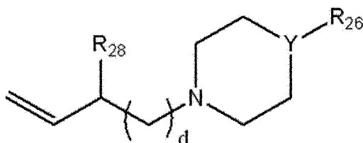
[Formula 16]
