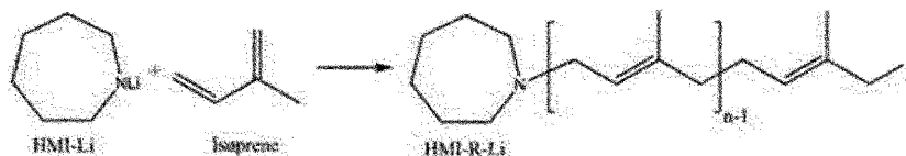
[Reaction Scheme 2]
