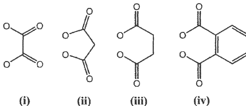
[Chemical Formula 12]
