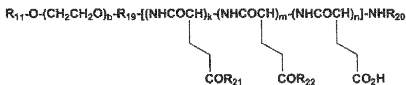
[Chemical Formula 6]
