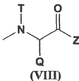
[Chemical Formula 8]
