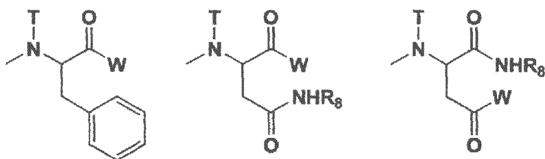
[Chemical Formula 10]
