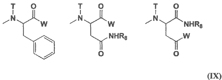
[Chemical Formula 9]
