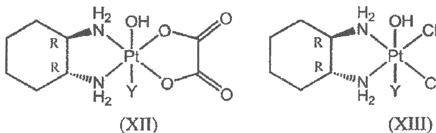
[Chemical Formula 13]
