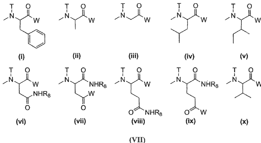
[Chemical Formula 7]
