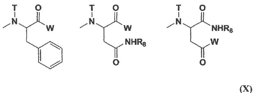
[Chemical Formula 10]
