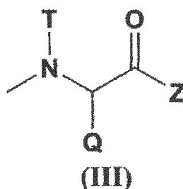
[Chemical Formula 3]
