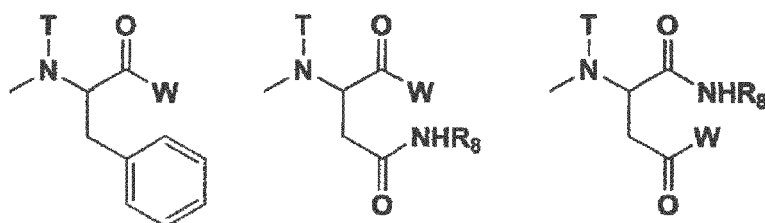
[Chemical Formula 9]
