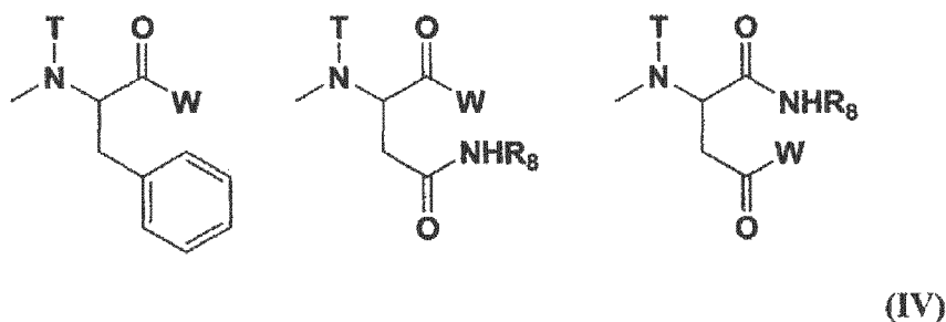
[Chemical Formula 4]
