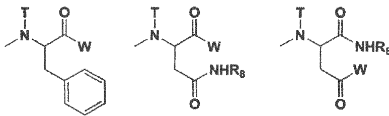
[Chemical Formula 4]
