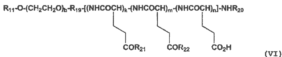
[Chemical Formula 6]
