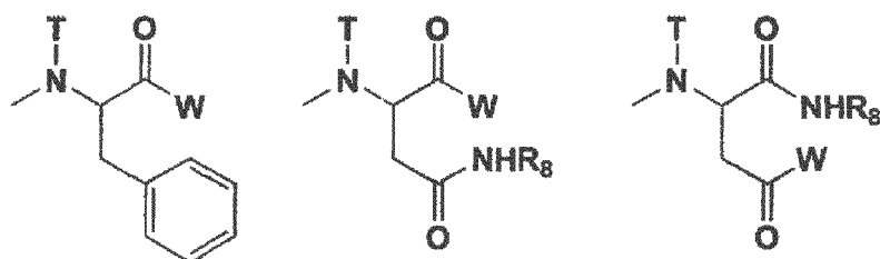
[Chemical Formula 5]
