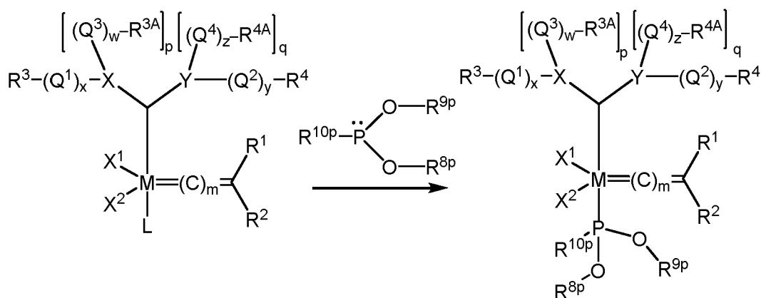
Formula (IIIS)
