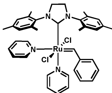
trans C727
