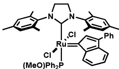
trans-C885
