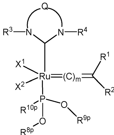
Formula (VII)
