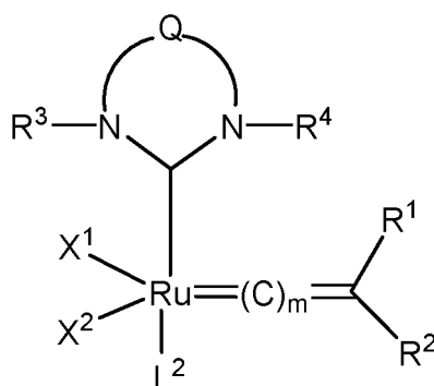
Formula (V)
