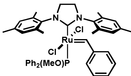
trans-C785
