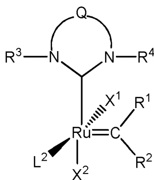
Formula (Vb)
