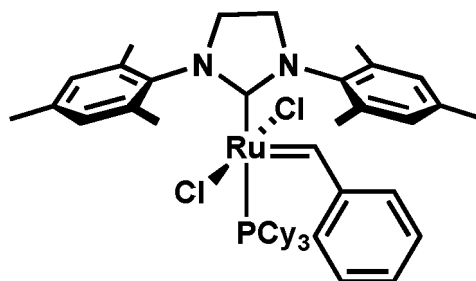
trans-C848
