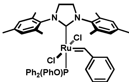
trans-C847
