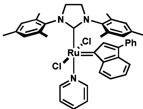
trans-C748
