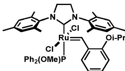
trans-C843
