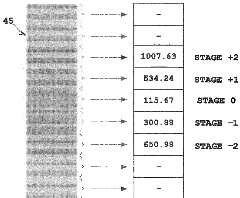
Fig.13 (a) SCAN IMAGE DATA
