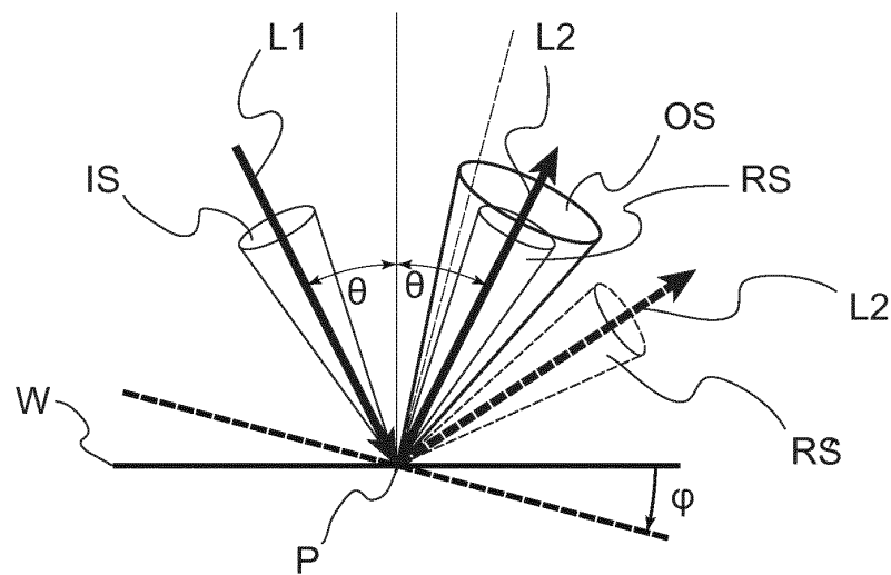
(b) Change in solid angle of reflected light and change in inclusive relation between solid angle of reflected light and observation solid angle
