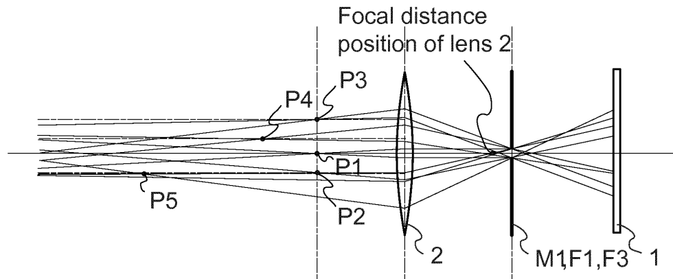
(c) When first shielding mask has a certain size and is located nearer to light source surface than focal distance position
