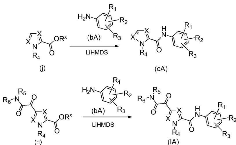
Scheme 3A
