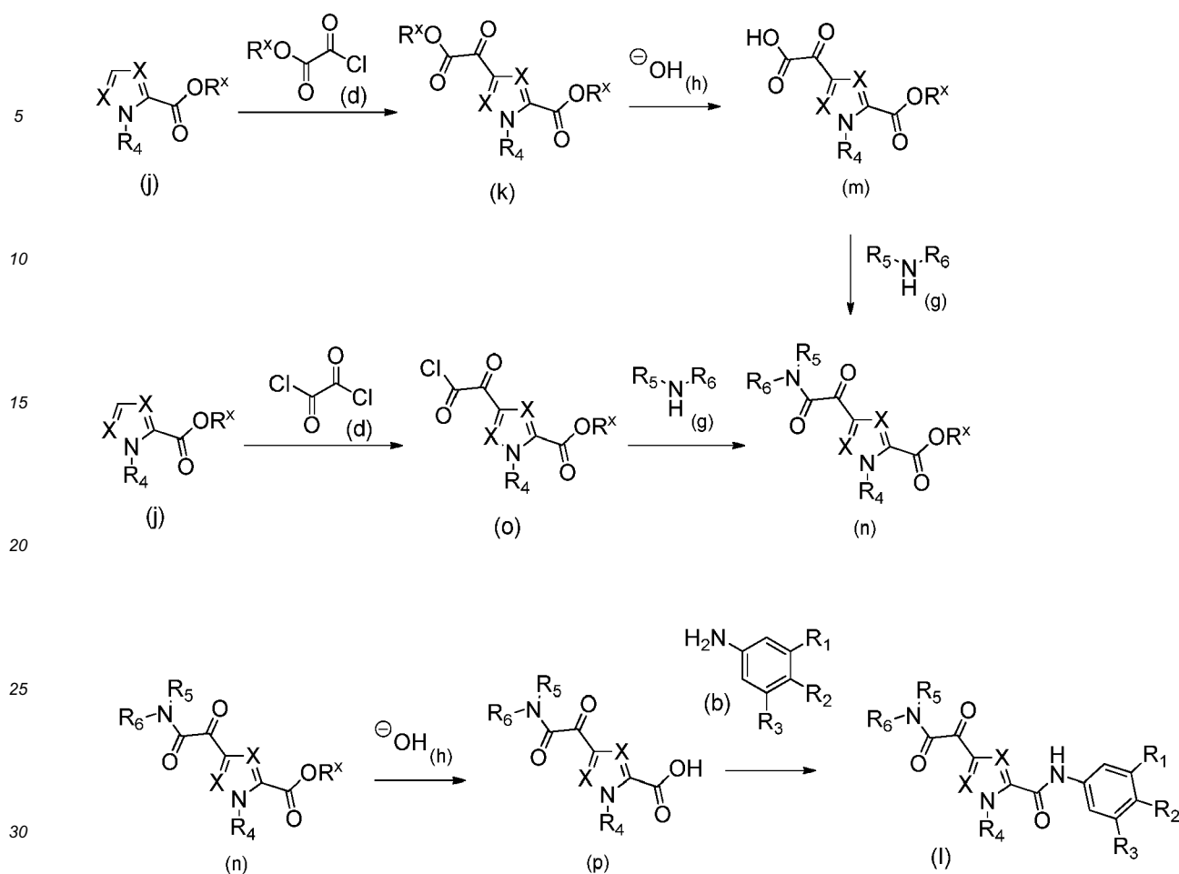
Scheme 2
