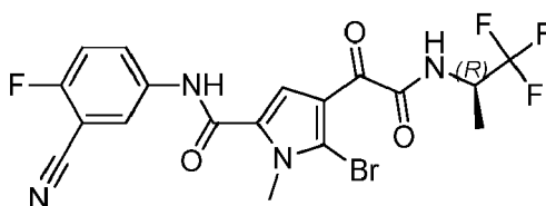
Compound 26 : 3-bromo-N-(3-cyano-4-fluoro-phenyl)-1-methyl-4-[2-oxo-2-[(1R)-2,2,2-trifluoro-1-methyl-ethyl]amino]acetyl]pyrrole-2-carboxamide
