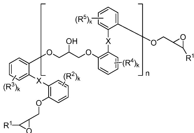
[Chemical compound 1]
