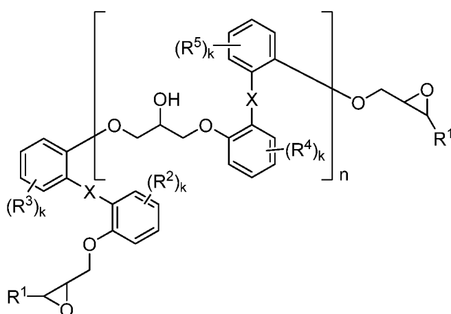
[Chemical compound 1]
