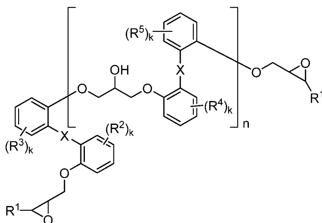
[Chemical compound 3]
