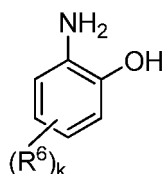
[Chemical compound 7]
