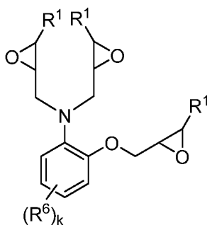
[Chemical compound 2]
