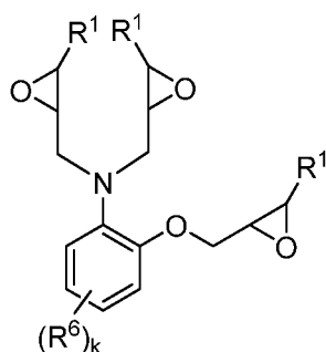
[Chemical compound 2]
