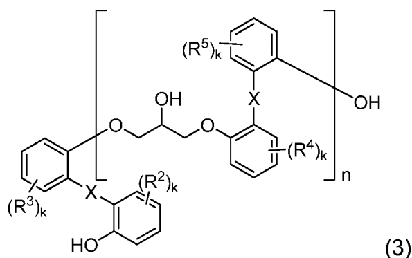
[Chemical compound 5]
