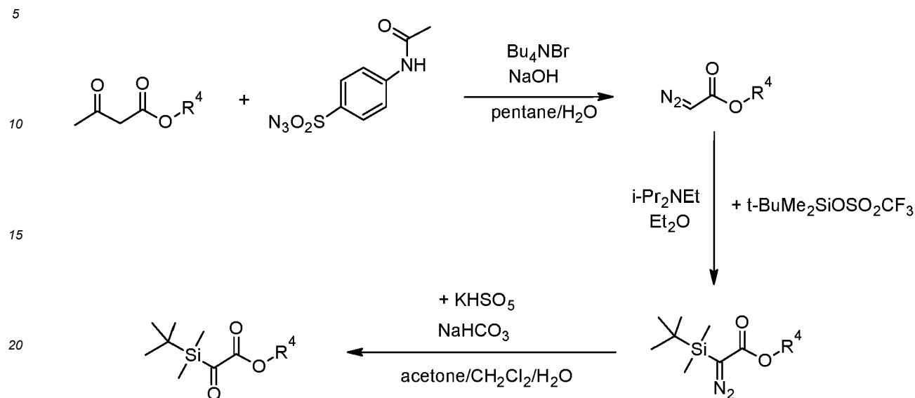
Scheme 2: Preparation of silylglyoxylates
