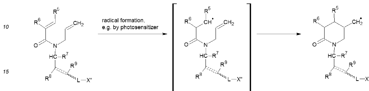
Scheme 7: Intramolecular cyclopolymerization of coinitiator compound of formula (IV)
