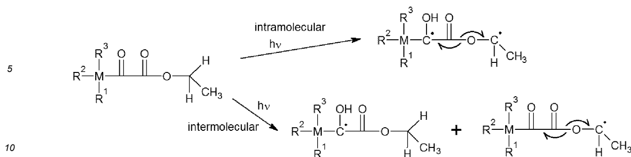
Scheme 6: hydrogen abstraction (intra- or intermolecular)
