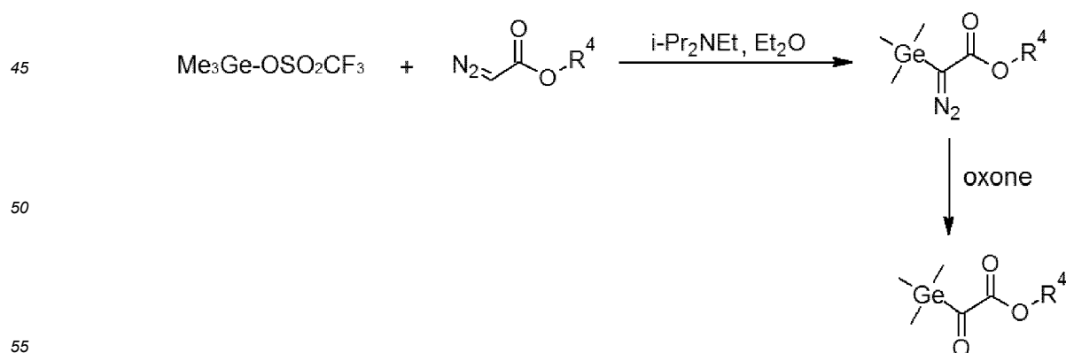
Scheme 3: Preparation of germlyglyoxylates
