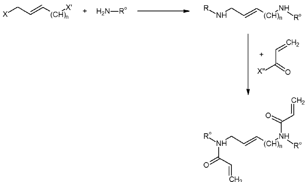
Scheme 8: Exemplary synthesis route for preparing coinitiator compound of formula (IV)
