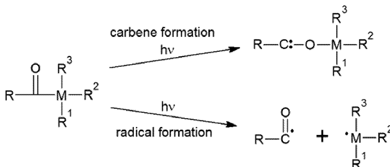
Scheme 4: carbene formation versus radical formation
