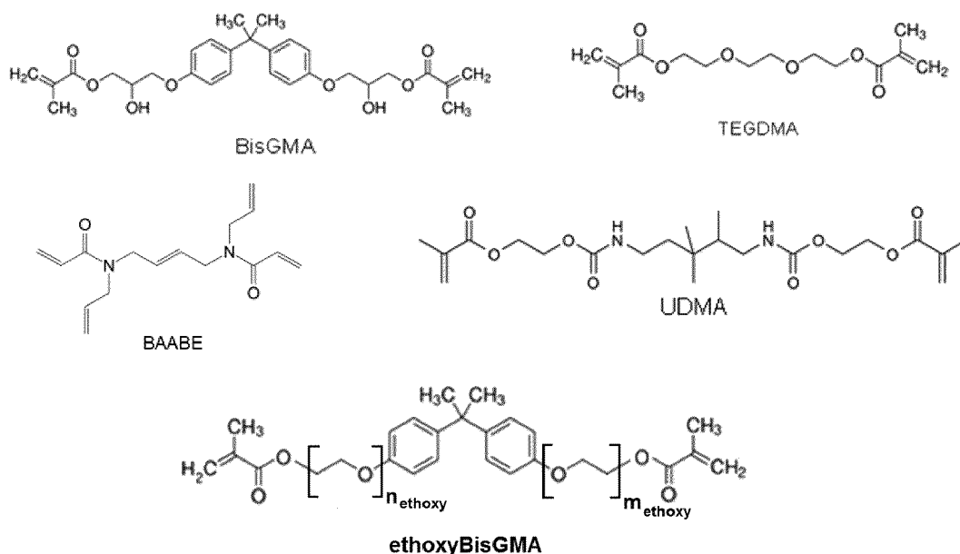
Scheme 9. Chemical structures of compounds applied in the photopolymerisation testings
