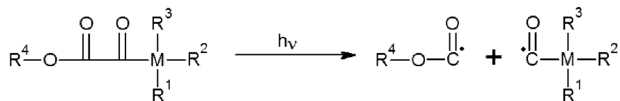
Scheme 5: cleavage of -O-C(=O)-C(=O)- moiety of a glyoxylate
