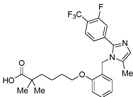
Scheme:
