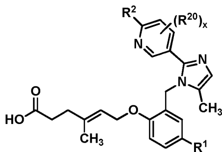
(IIb); or
