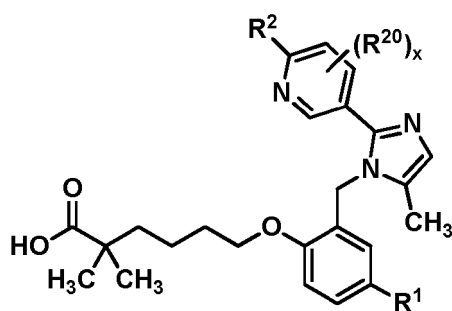
(IIIb);
