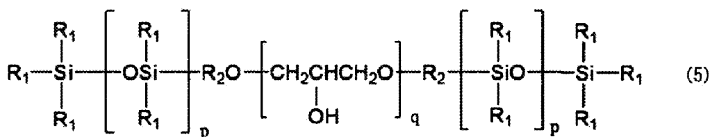
[Chemical Formula 4]
