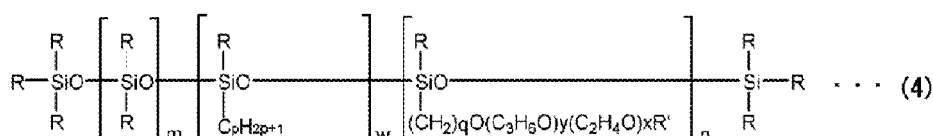
[Chemical Formula 3]
