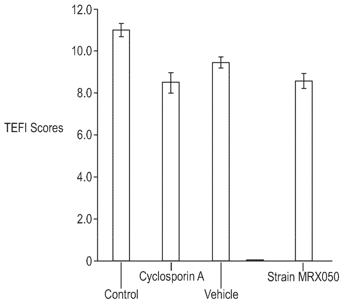
FIG. 2 TEFI scores
