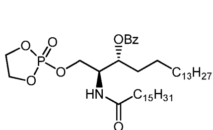
N-palmitoyl 3-O-Benzoyl- 1-O-(2-oxo-1,3,2-dioxaphospholan) D-erythro-dihydrosphingosine Compound VIIIId ;
