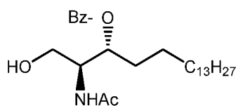
3-O-Benzoyl-D-erythro-dihydroceramide Compound VIIe ;
