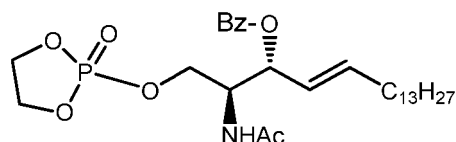
3-O-Benzoyl- D -erythro-1-O-(2-oxo-1,3,2-dioxaphospholan)-ceramide Compound Vf-Bz
