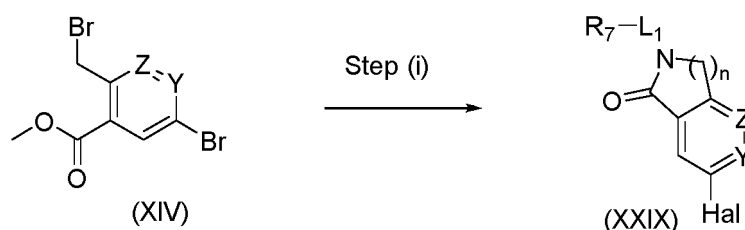
Scheme 12
