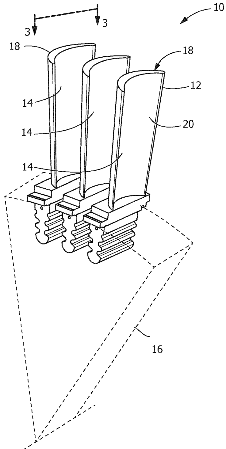
FIG. 2 (Prior Art)
