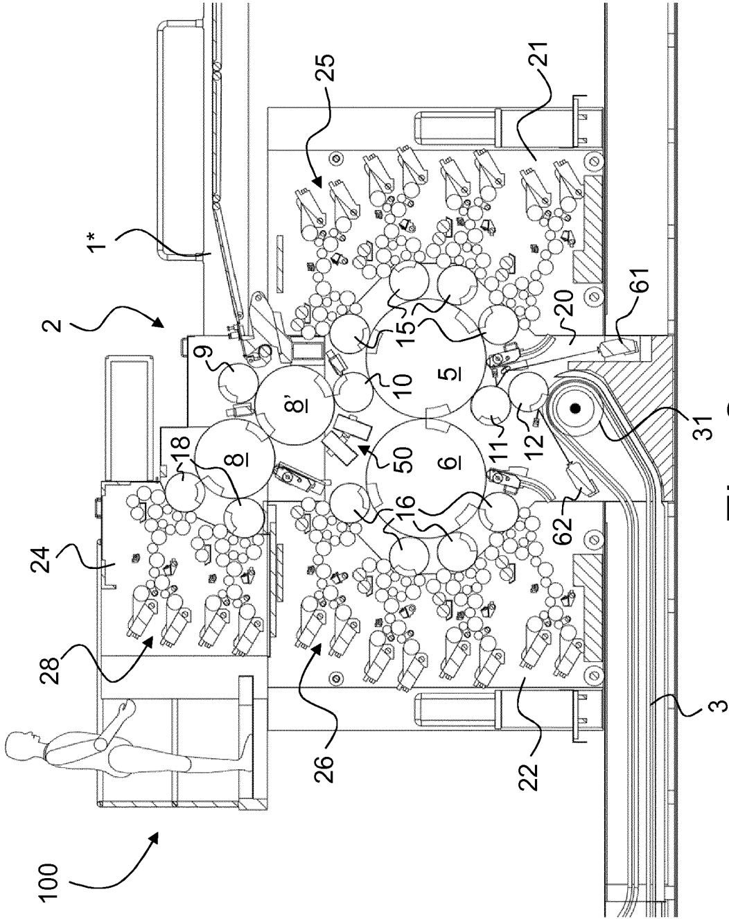
Fig. 2 (PRIOR ART)
