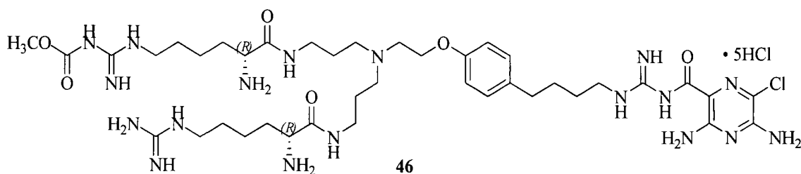
Scheme 8. The Preparation of the Hydrochloride Salt of (S)-3,5-diamino-N-(N-(4-(4-(2-((3-(2-amino-6-guanidinohexanamido)propyl)(3-aminopropyl)amino)ethoxy)phenyl)butyl)carbamimidoyl)-6-chloropyrazine-2-carboxamide-Compound 46
