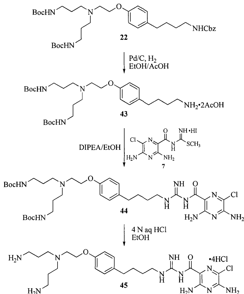
Scheme 7. The Preparation of the Hydrochloride Salt of 3,5-diamino-N-(N-(4-(4-(2-(bis(3-aminopropyl)amino)ethoxy)phenyl)butyl)carbamimidoyl)-6-chloropyrazine-2-carboxamide-Compound 45
