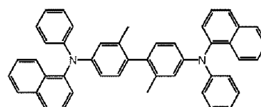
methylated NPB
