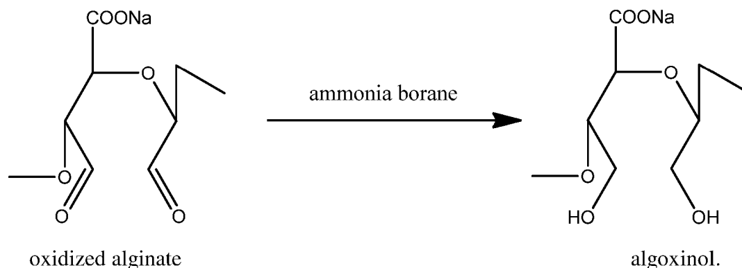
Scheme 2.
