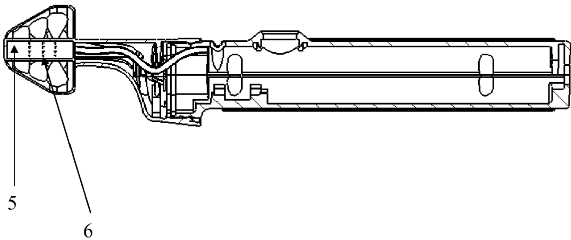
Cross-section A-A
