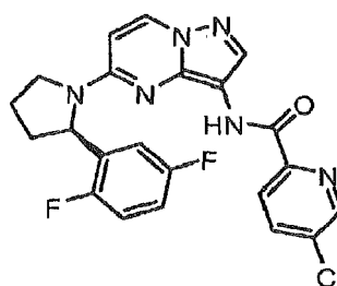
(R)-5-chloro-N-(5-(2-(2,5-difluorophenyl)pyrrolidin-1-yl)pyrazolo[1,5-a]pyrimidin-3-yl)picolinamide
