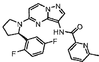
(R)-N-(5-(2-(2,5-difluorophenyl)pyrrolidin-1-yl)pyrazolo[1,5-a]pyrimidin-3-yl)-6-methylpicolinamide
