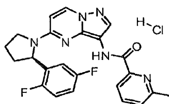
(R)-N-(5-(2-(2,5-difluorophenyl)pyrrolidin-1-yl)pyrazolo[1,5-a]pyrimidin-3-yl)-6-methylpicolinamide hydrochloride
