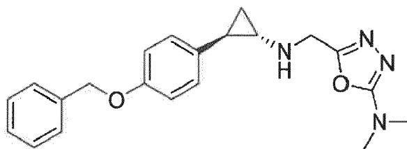
Example 27: 3-((((trans)-2-(4-(benzyloxy)phenyl)cyclopropyl)amino)methyl)-1,2,4-oxadiazol-5-amine
