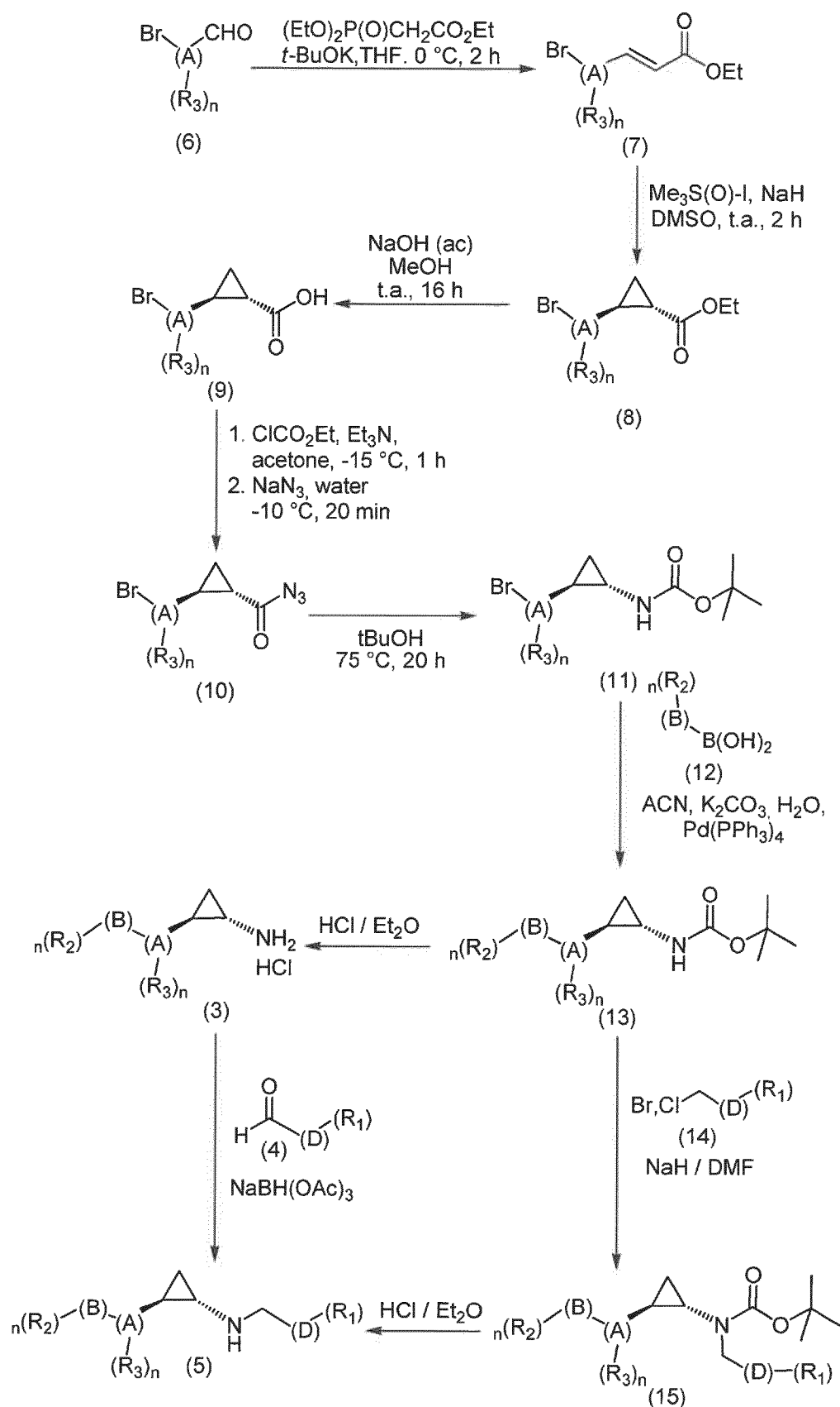
SCHEME 2: ACN (acetonitrile), DMSO (Dimethyl sulfoxide), THF (Tetrahydrofuran).
