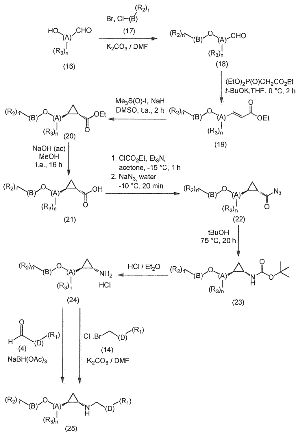
SCHEME 3: DMF (N,N-dimethylformamide), DMSO (Dimethyl sulfoxide), THF (Tetrahydrofuran).
