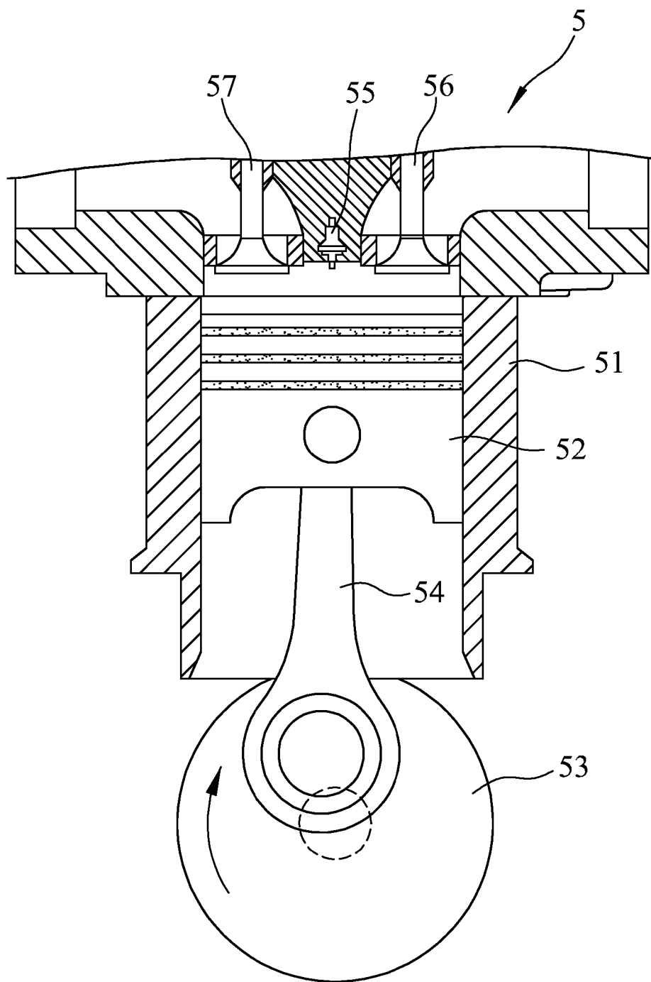
FIG.7 PRIOR ART
