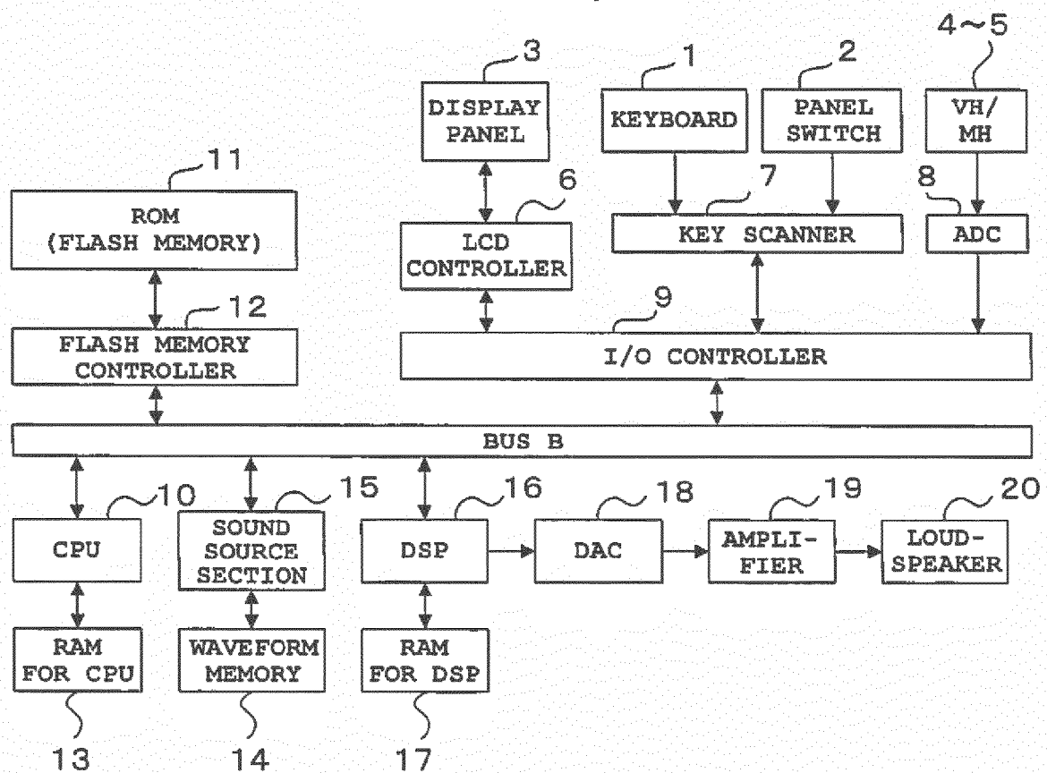
FIG. 1B BLOCK DIAGRAM
