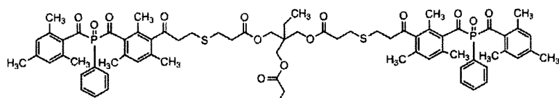
Compound B2-(1)
