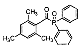
Compound C1-(1)
