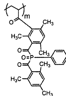
Compound B2-(10)
