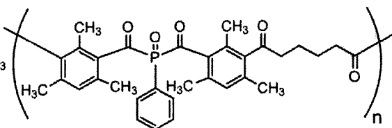
Compound B1-(10)
