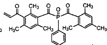
Compound B1-(3)
