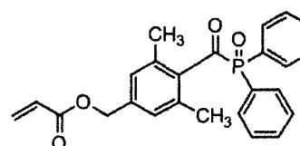
Compound C1-(3)
