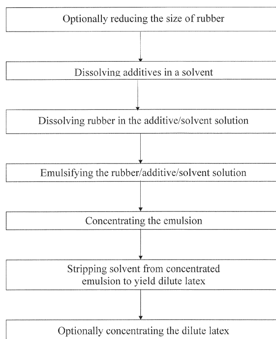
FIGURE 1 AQUEOUS ELASTOMER DISPERSION PREPARATION FLOWCHART
