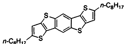
Specific Low Molecular Weight Compound (2)
