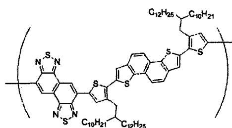
Specific Polymer Compound (2) Mw = 77,000
