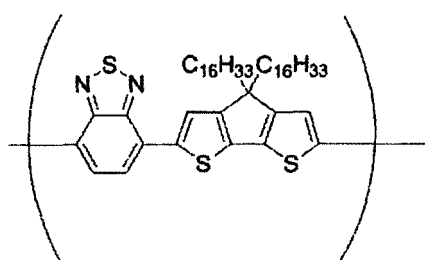
Comparative Polymer Compound (3) Mw = 48,000
