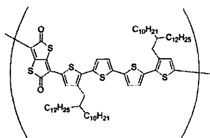
Specific Polymer Compound (1) Mw = 61,000
