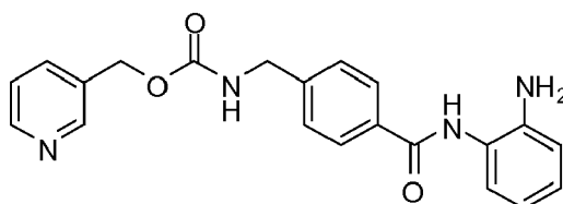
Chemical structure of entinostat
