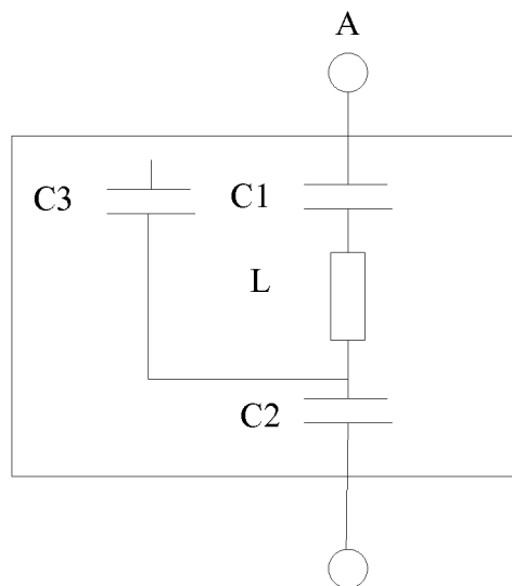
Output end of a matching circuit
