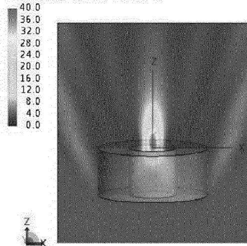
XYZ Poynting vector [ \text{mW}/\text{m}^2 ]
