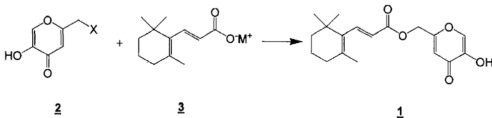
[Reaction Scheme 1]
