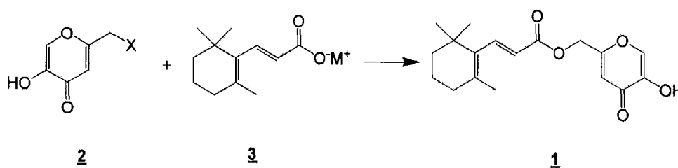
[Reaction Scheme 1]
