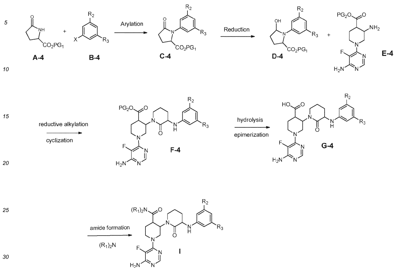
Scheme 4
