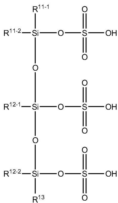
[Chemical Formula 233]
