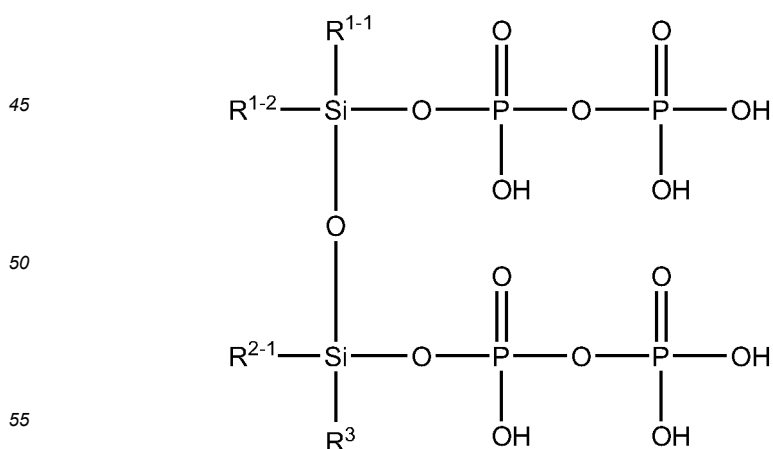
[Chemical Formula 203]
