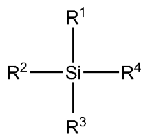
[Chemical Formula 10]
