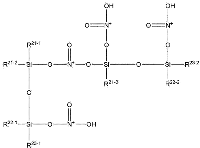
[Chemical Formula 267]
