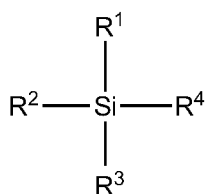
[Chemical Formula 300]
