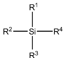
[Chemical Formula 10]
