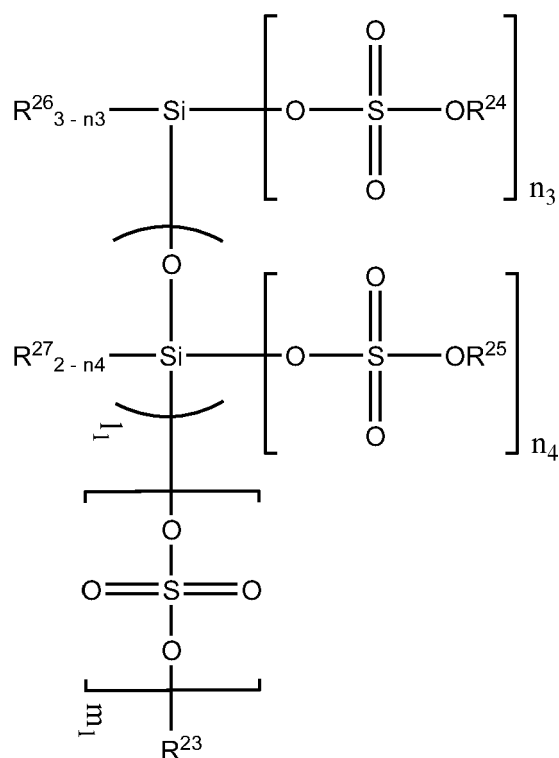
[Chemical Formula 250]
