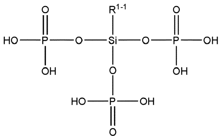
[Chemical Formula 53]
