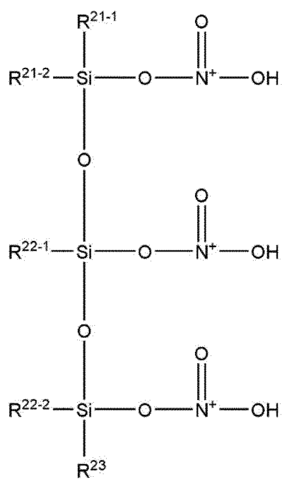
[Chemical Formula 263]
