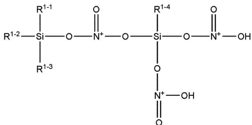
[Chemical Formula 77]
