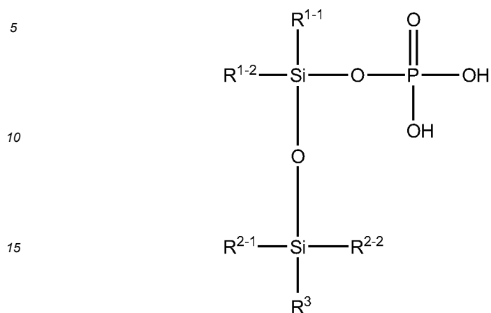
[Chemical Formula 201]
