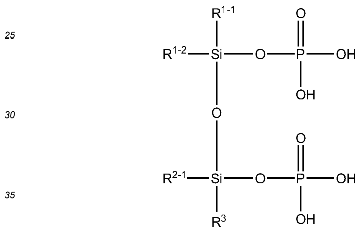
[Chemical Formula 202]
