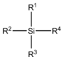
[Chemical Formula 10]
