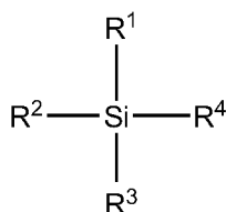
[Chemical Formula 300]
