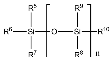
[Chemical Formula 20]
