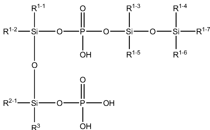
[Chemical Formula 206]
