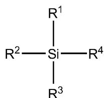
[Chemical Formula 10]
