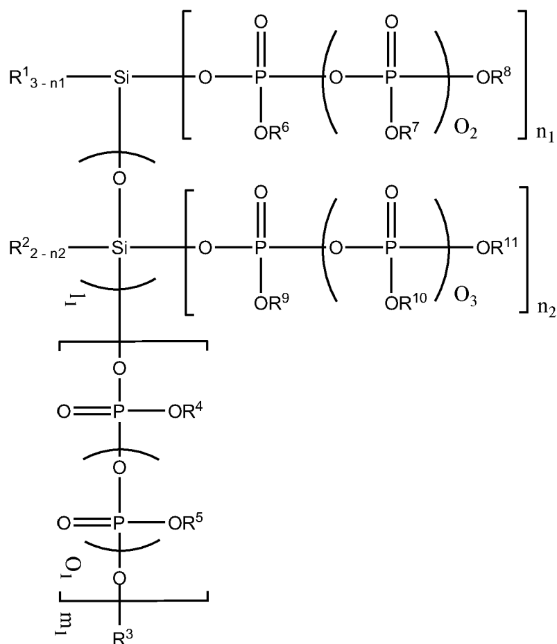
[Chemical Formula 200]
