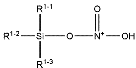
[Chemical Formula 67]
