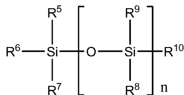
[Chemical Formula 20]
