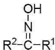
[Chemical Formula 400]
