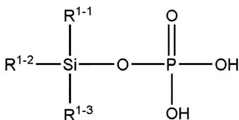
[Chemical Formula 51]
