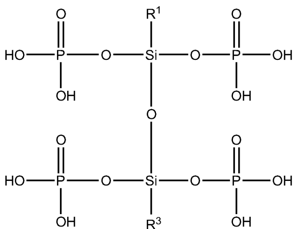
[Chemical Formula 205]
