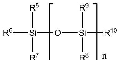
[Chemical Formula 20]
