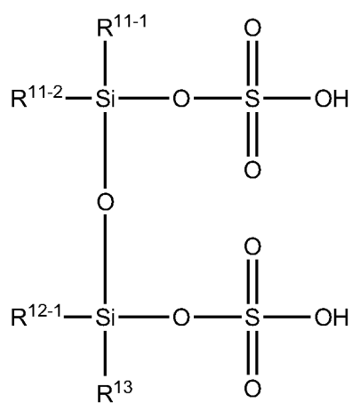
[Chemical Formula 232]
