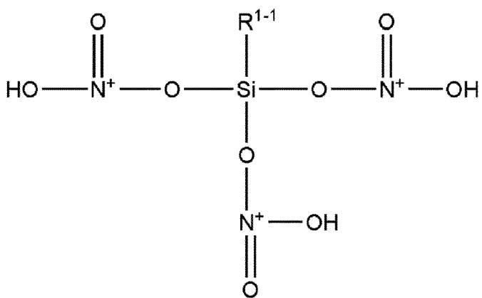
[Chemical Formula 73]
