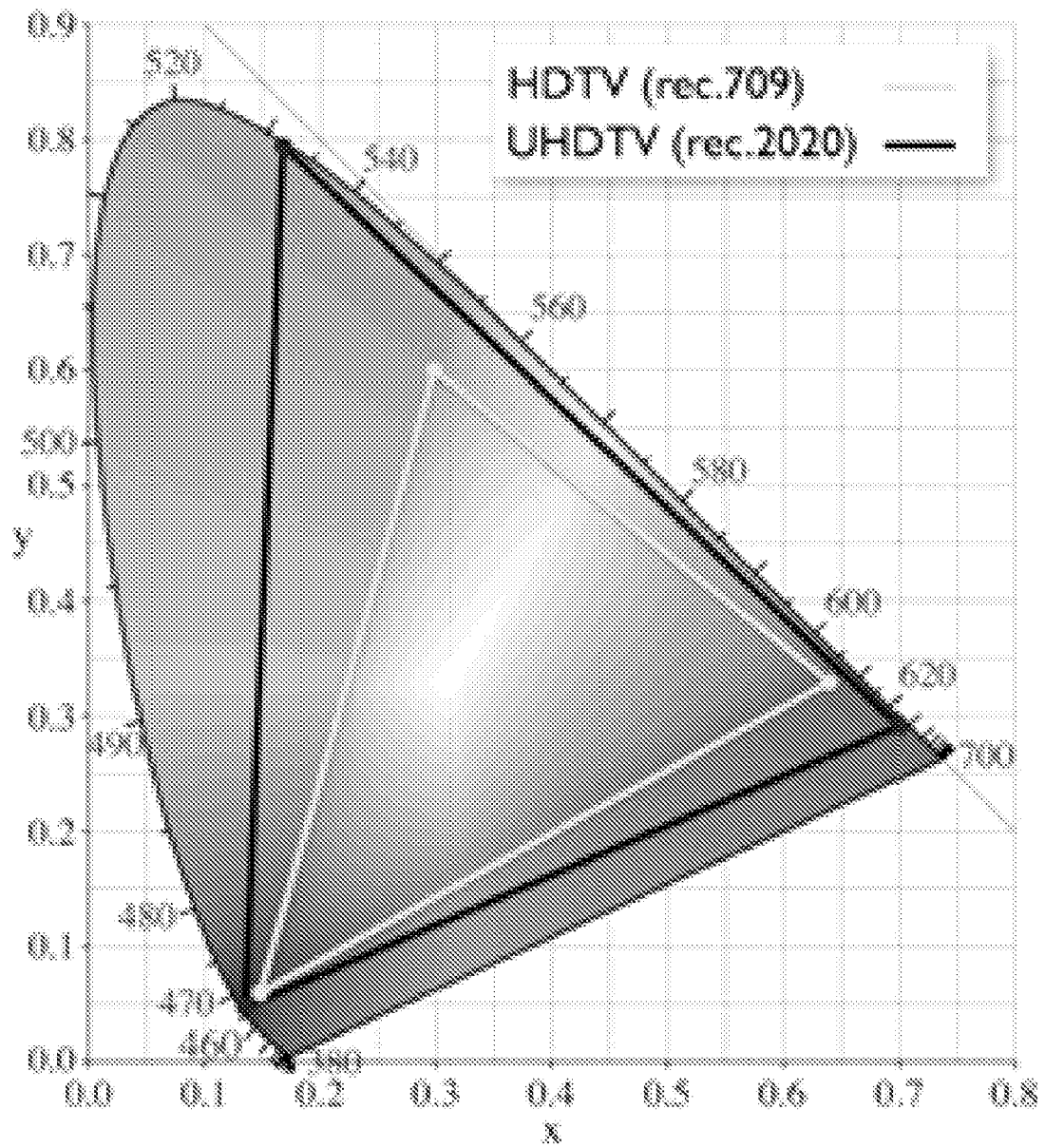
UHD TV vs HDTV Color Gamuts
