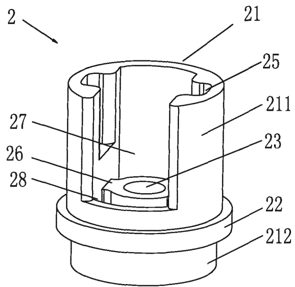
FIG. 2(Prior Art)
