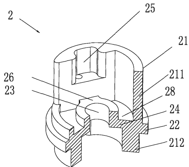
FIG. 3(Prior Art)
