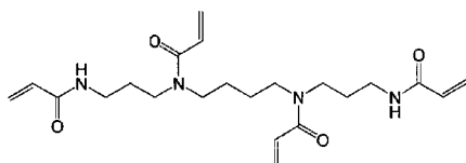
Compound (a1-7)
