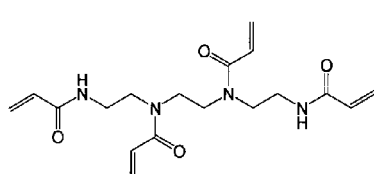
Compound (a1-5)
