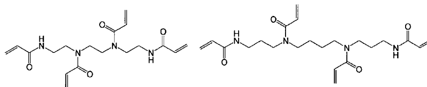
Compound (a1-7)
