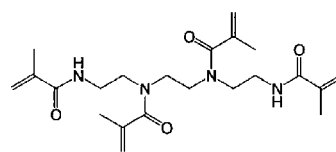
Compound (a1-6)
