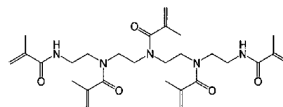
Compound (a1-10)
