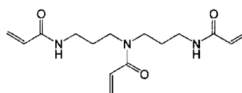
Compound (a1-3)
