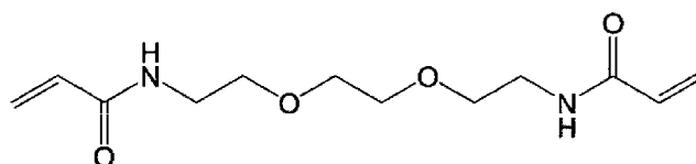
Compound (a2-21)
