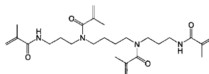
Compound (a1-8)
