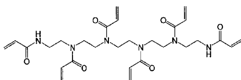
Compound (a1-11)
