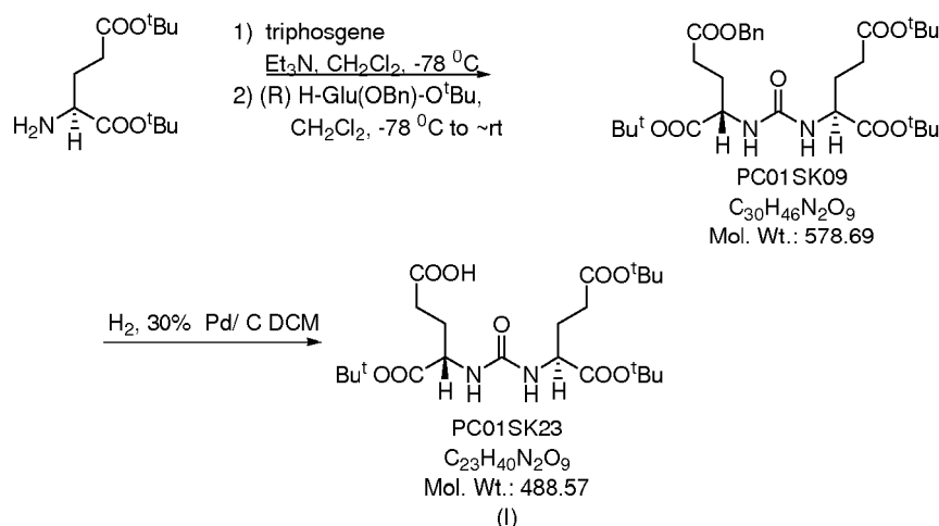
Scheme 2.1
