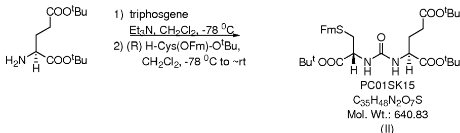
Scheme 2.2
