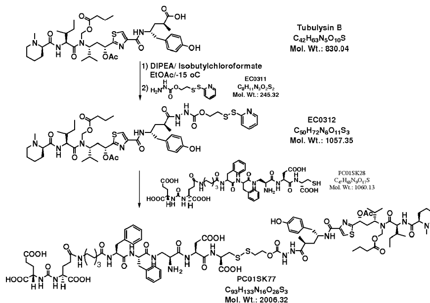
Scheme 6.4
