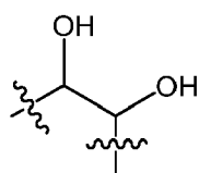
1,2-OH Configuration
