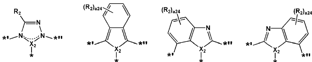
Formula Cy2-36
