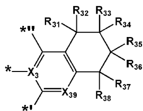
Formula Cy3-10
