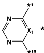
Formula Cy1(21)
