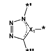
Formula Cy1-29
