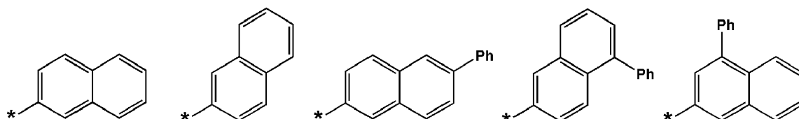
Formula 10-87
