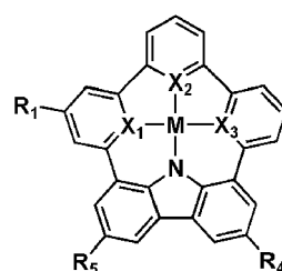
Formula 1-7
