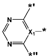
Formula Cy1(21)
