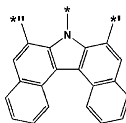
Formula Cz(21)
