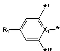
Formula Cy1(3)
