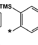
Formula 10-47
