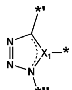
Formula Cy1-33
