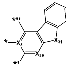
Formula Cy3(26)
