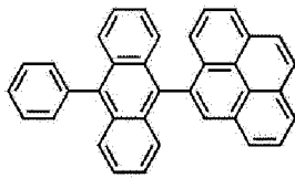
H6
