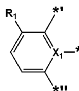
Formula Cy1(4)
