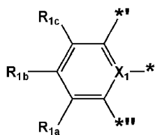
Formula Cy1(8)
