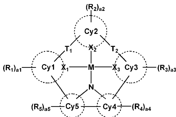
Formula 1
