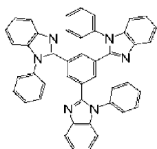
TPBi
