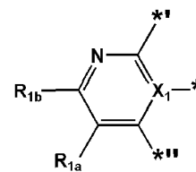
Formula Cy1(20)
