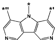
Formula Cz(9)
