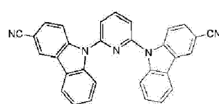
Compound H51
