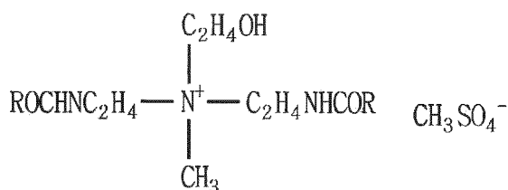
[Chemical Formula 5]
