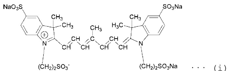
[Chemical Formula 6]
