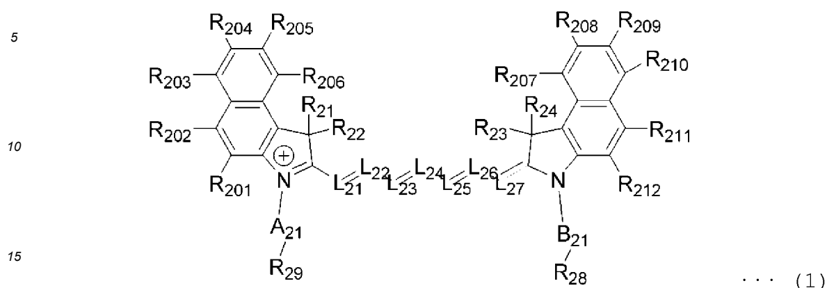
[Chemical Formula 1]
