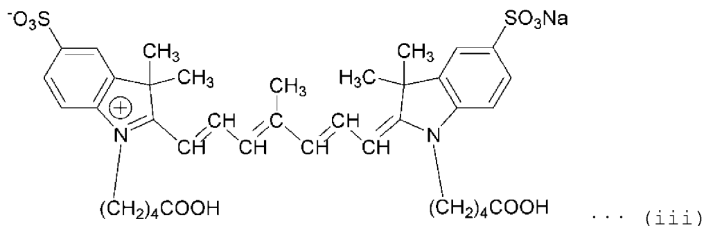
[Chemical Formula 7]
