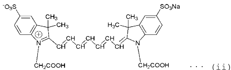
[Chemical Formula 6]
