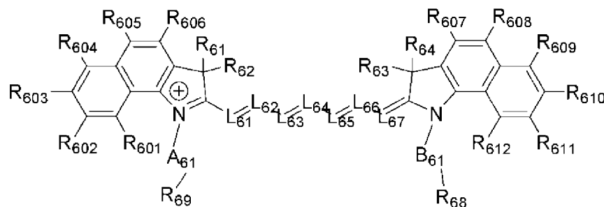
[Chemical Formula 3]
