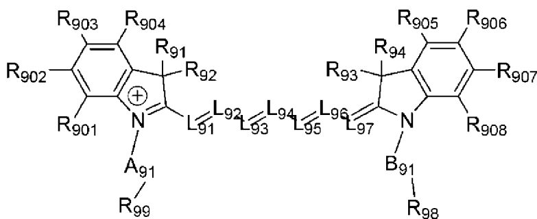
[Chemical Formula 4]
