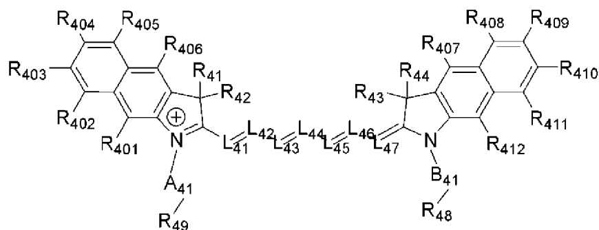
[Chemical Formula 2]
