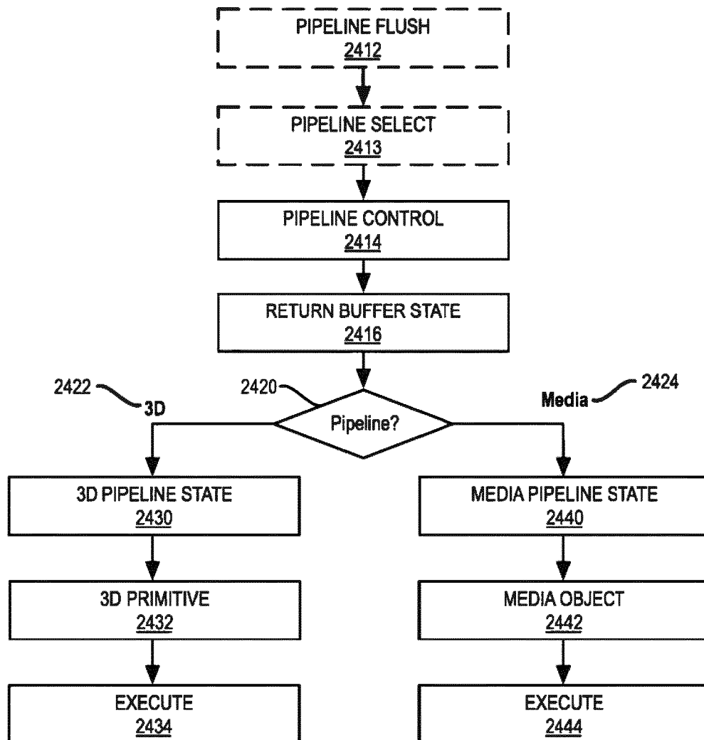
GRAPHICS PROCESSOR COMMAND SEQUENCE 2410
