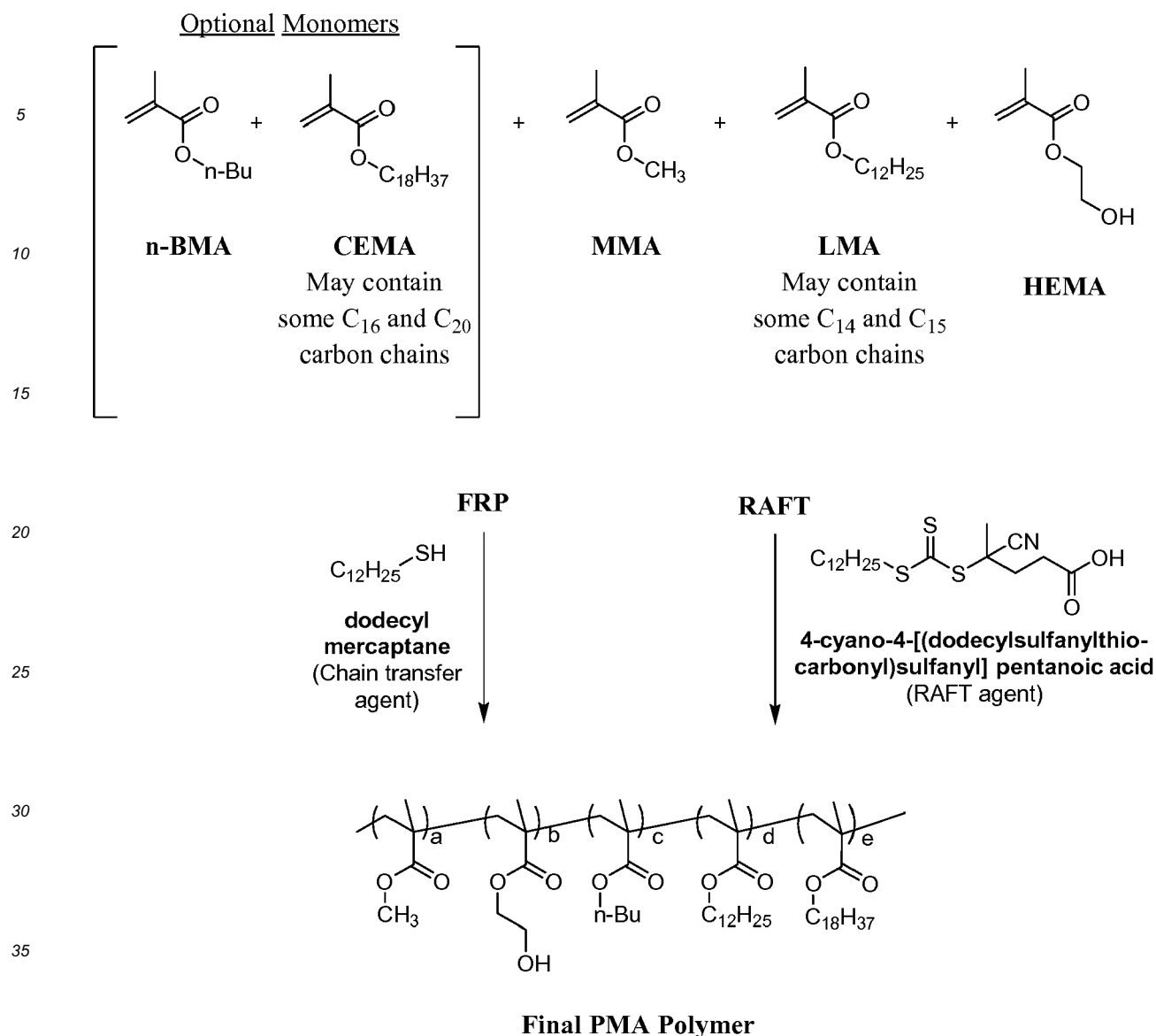
Scheme 1: General procedure for PMA synthesis via the free radical polymerization (FRP) pathway and the reversible addition-fragmentation chain transfer (RAFT) pathway.
